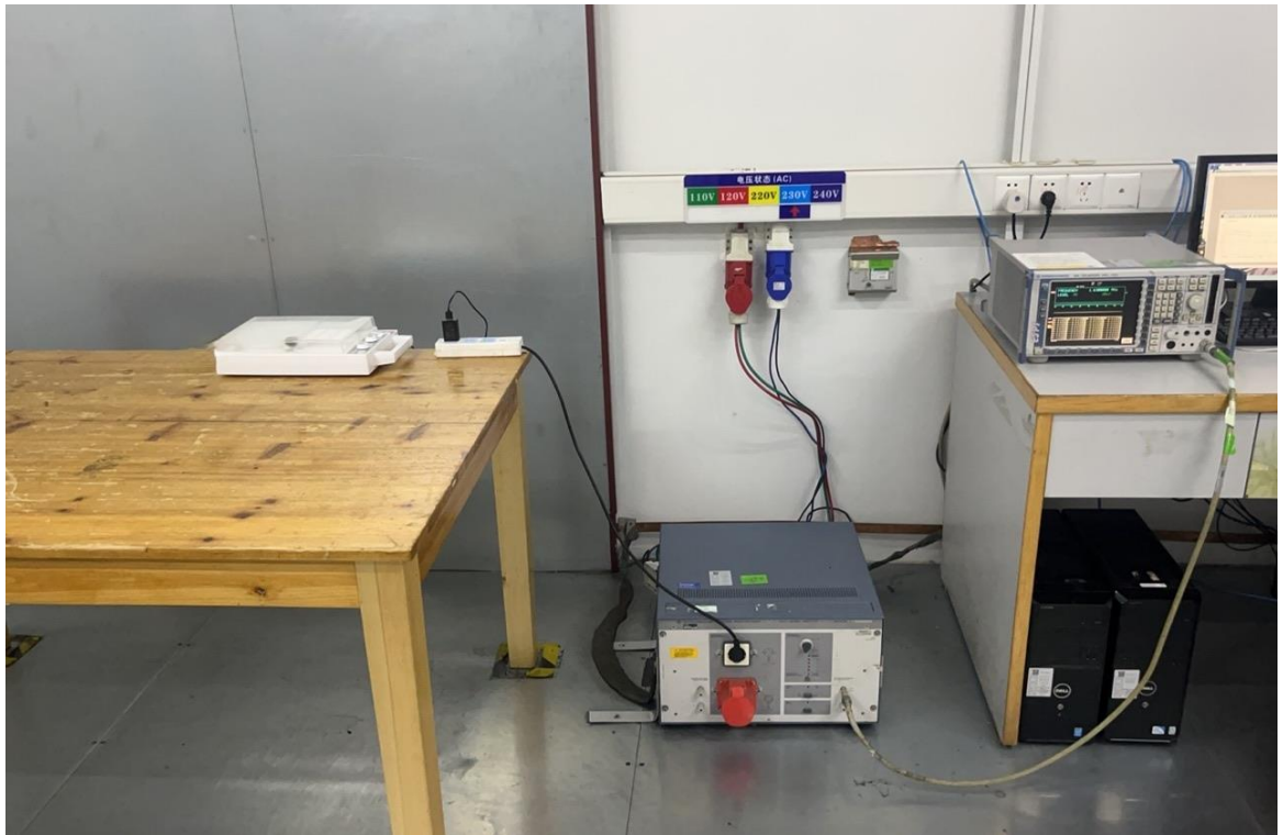
AC POWER LINE CONDUCTED TEST SETUP
