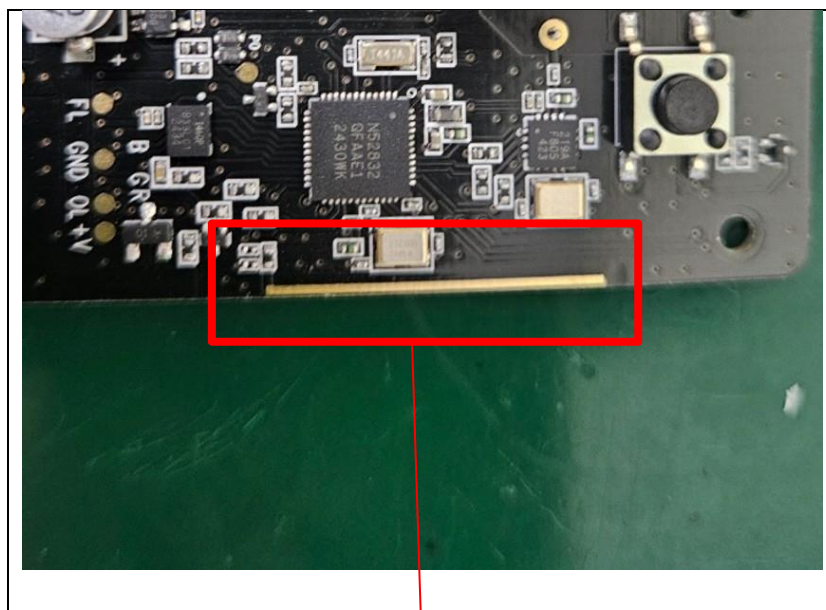
Bluetooth Antenna
