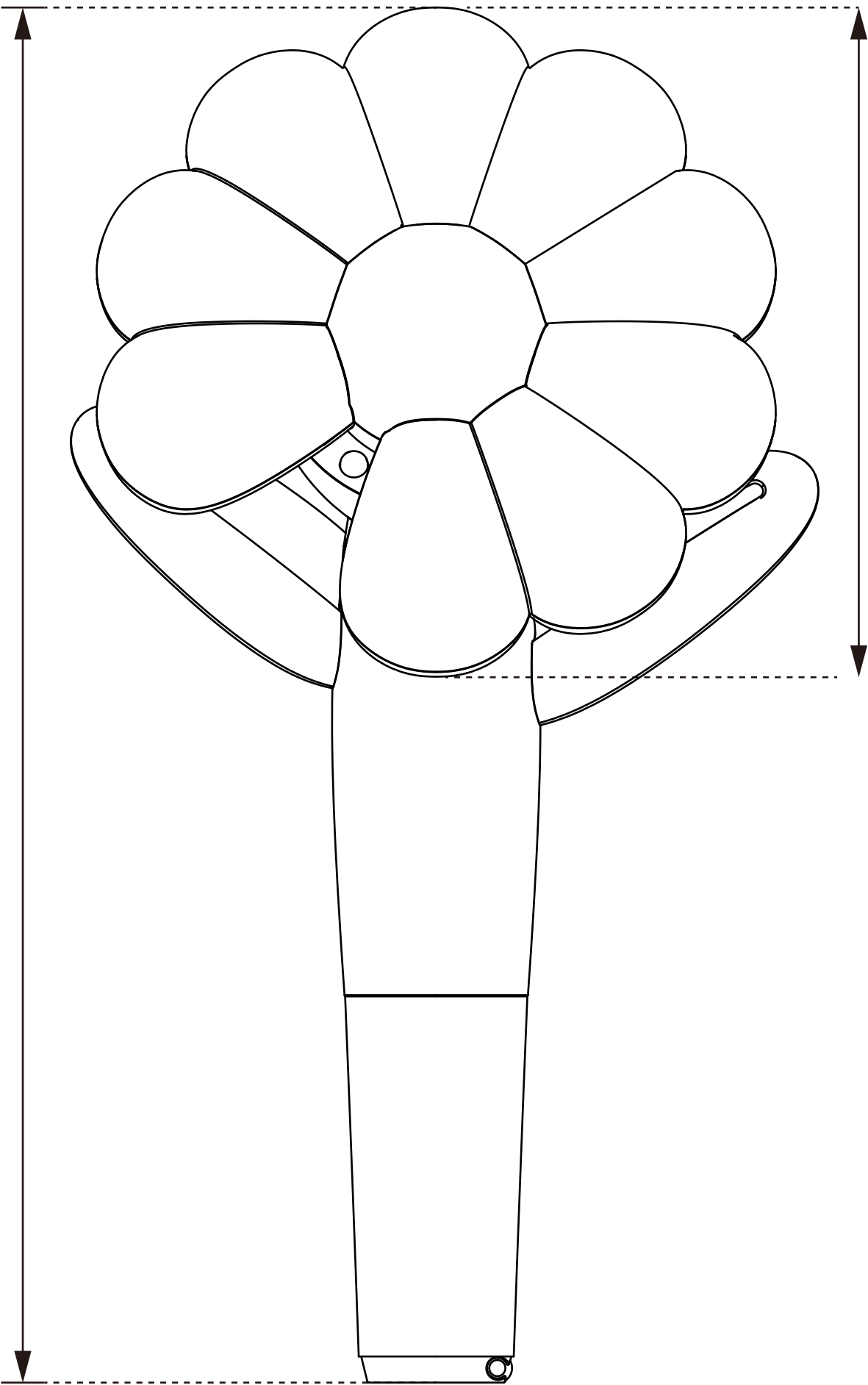
FRONT
