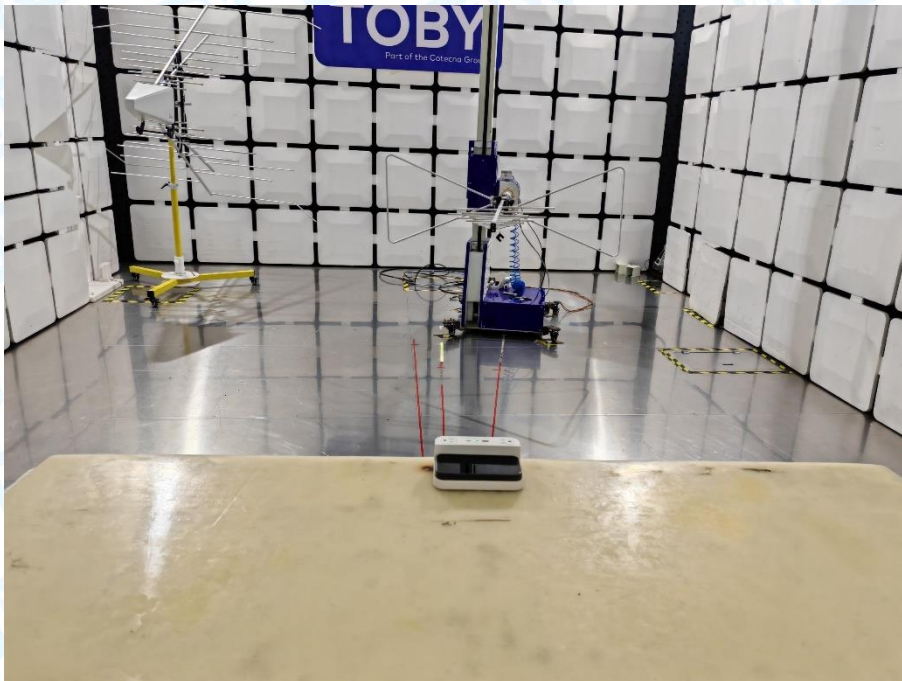
Photo of Setup for Radiated Emission (Below 30MHz)
