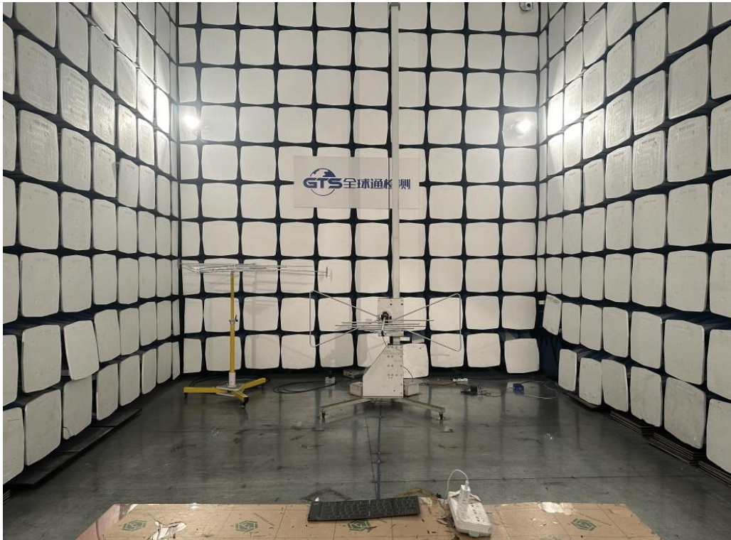
Photo of Radiated Emissions Measurement
