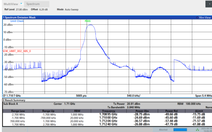
Band66-1.4MHz-QPSK-132665-1RB#5
