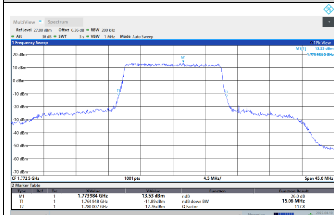
Band66-15MHz-16QAM-132322-75RB#0
