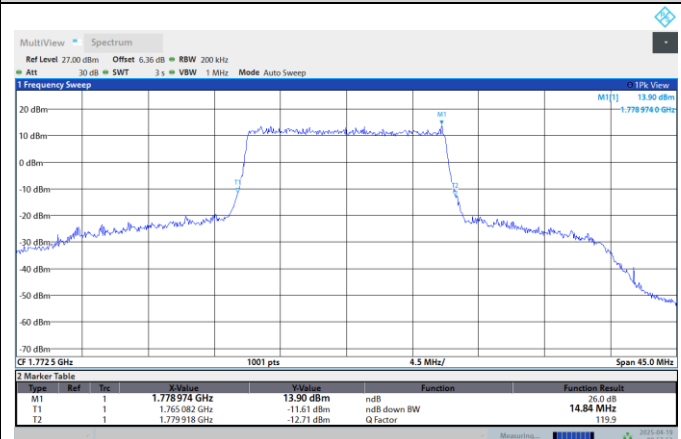
Band66-15MHz-64QAM-132322-75RB#0
