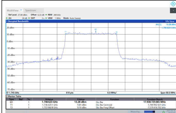
Band66-20MHz-16QAM-132072-100RB#0
