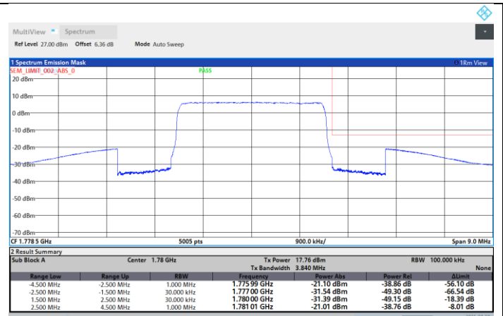
Band66-3MHz-64QAM-131987-15RB#0
