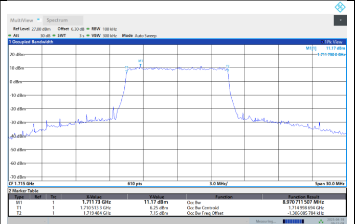
Band66-10MHz-64QAM-132622-50RB#0
