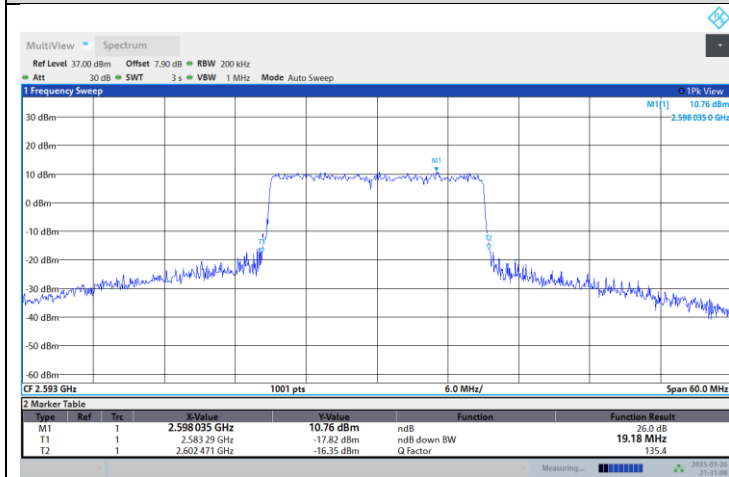
Band41-20MHz-64QAM-40620-100RB#0
