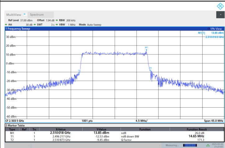
Band41-15MHz-16QAM-41515-75RB#0
