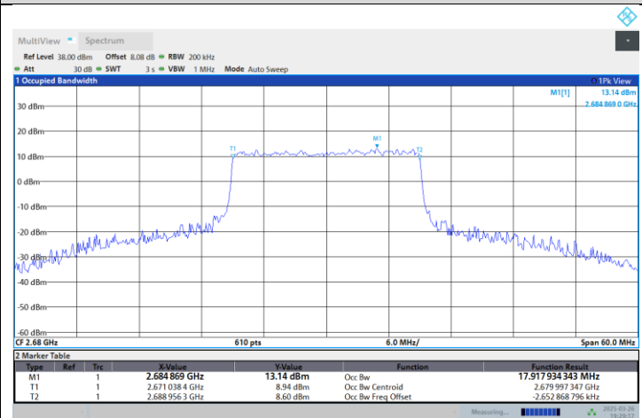
Band41-20MHz-16QAM-40620-100RB#0
