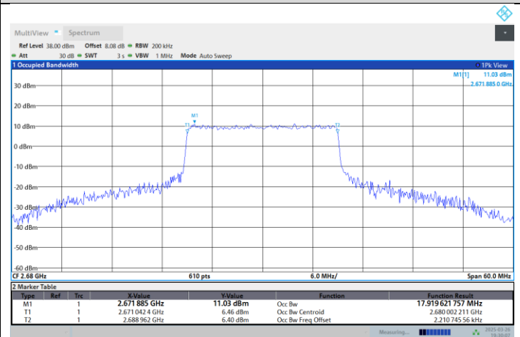
Band41-20MHz-64QAM-41490-100RB#0
