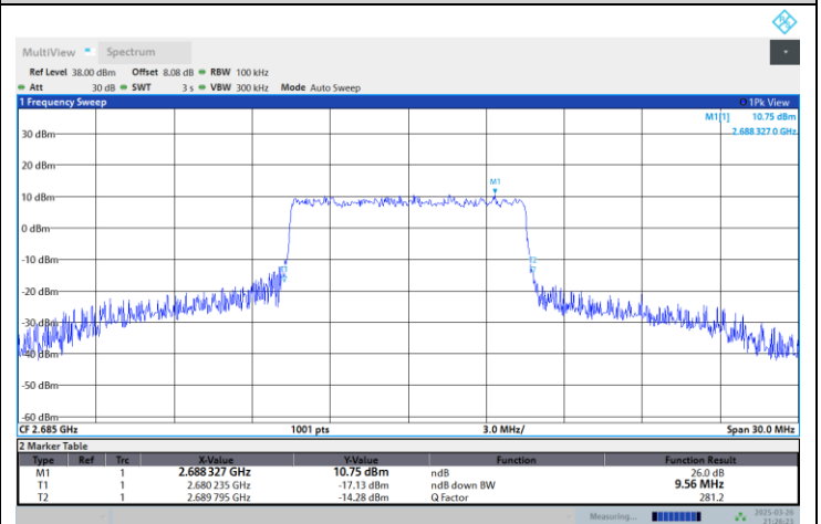
Band41-15MHz-QPSK-40620-75RB#0
