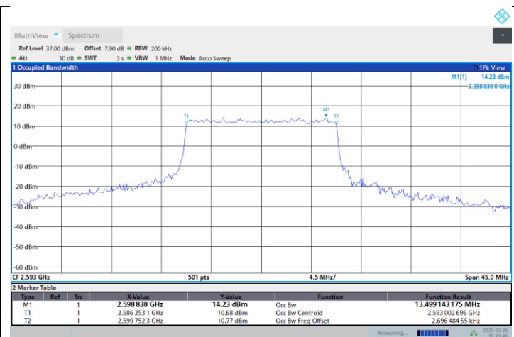
Band41-15MHz-16QAM-39725-75RB#0
