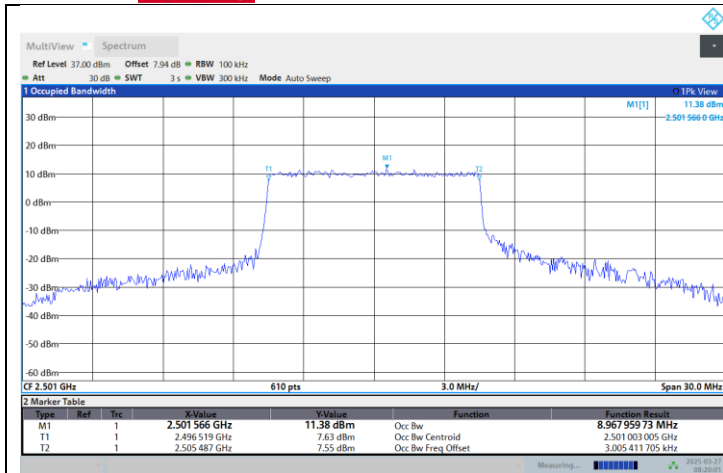
Band41-10MHz-16QAM-41540-50RB#0
