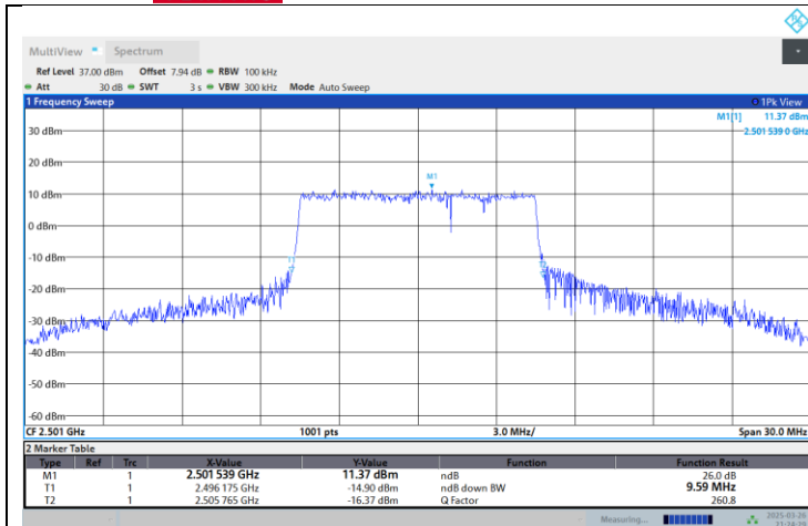
Band41-10MHz-16QAM-41540-50RB#0
