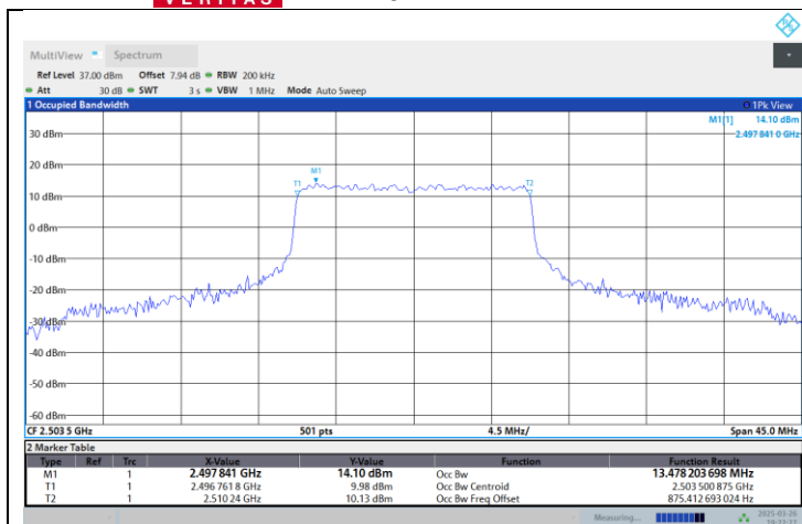
Band41-15MHz-QPSK-41515-75RB#0
