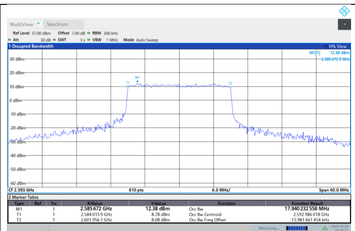
Band41-20MHz-64QAM-39750-100RB#0
