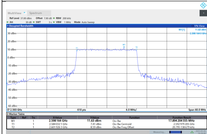
Band41-20MHz-64QAM-40620-100RB#0
