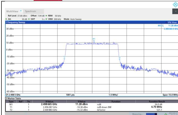
Band41-5MHz-64QAM-41565-25RB#0
