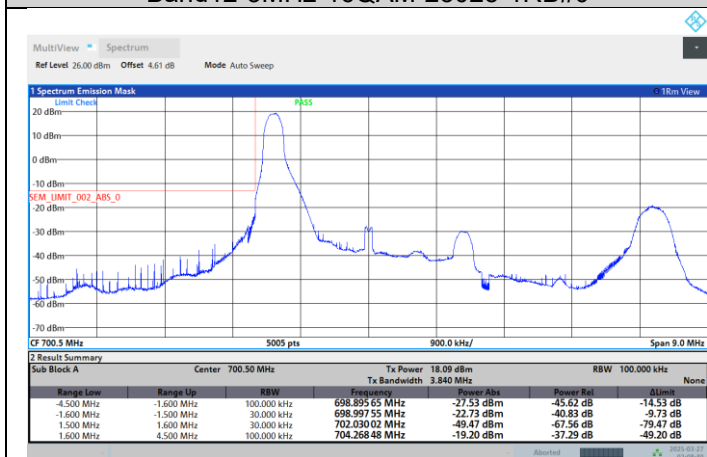
Band12-3MHz-16QAM-23165-1RB#14
