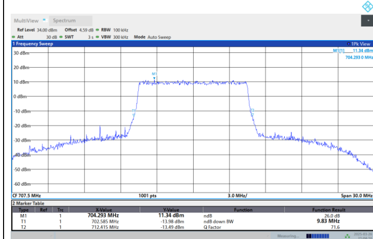
Band12-10MHz-64QAM-23095-50RB#0
