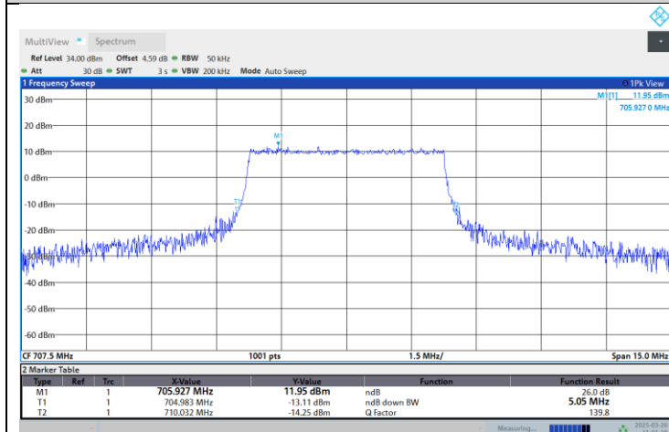
Band12-5MHz-64QAM-23035-25RB#0
