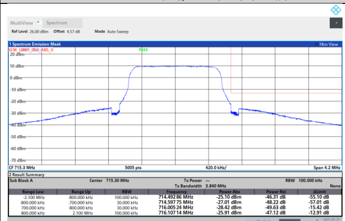
Band12-3MHz-QPSK-23025-15RB#0
