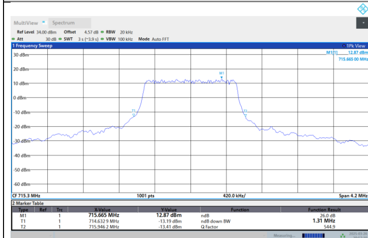
Band12-3MHz-QPSK-23095-15RB#0
