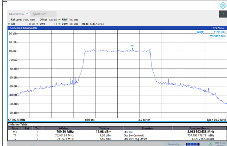
Band12-10MHz-64QAM-23095-50RB#0
