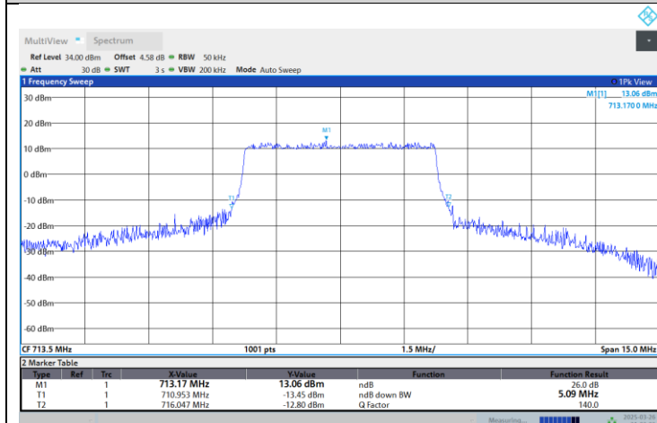
Band12-5MHz-16QAM-23095-25RB#0
