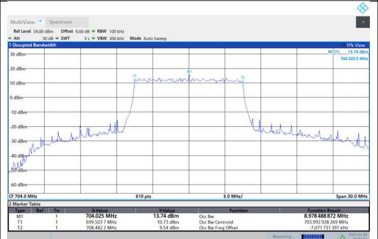
Band12-10MHz-QPSK-23130-50RB#0
