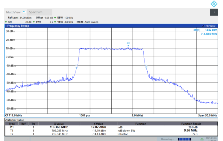
Band12-10MHz-64QAM-23130-50RB#0
