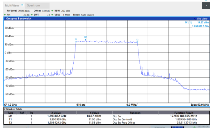
Band2-20MHz-64QAM-19100-100RB#0
