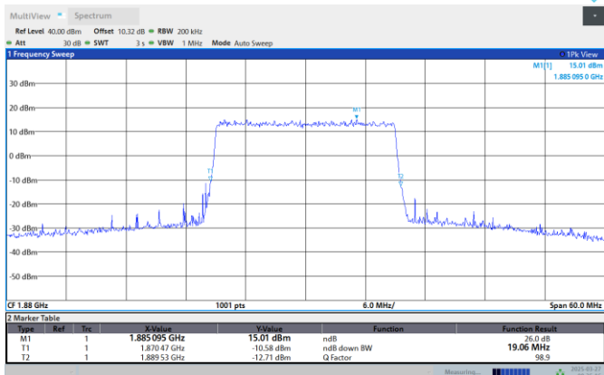
Band2-20MHz-64QAM-18900-100RB#0
