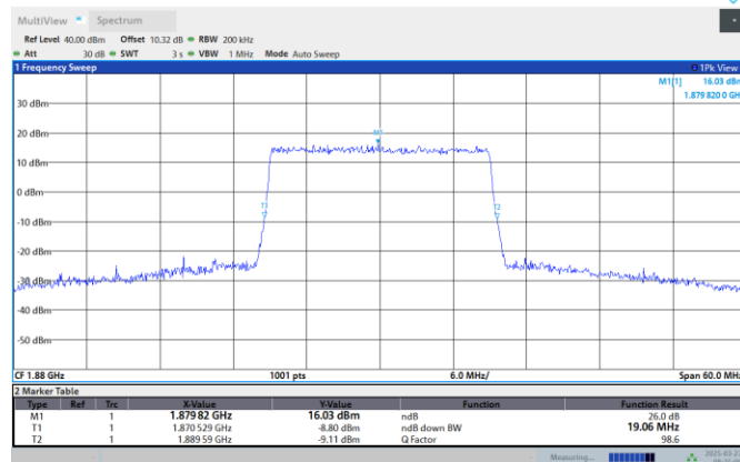
Band2-20MHz-64QAM-18700-100RB#0
