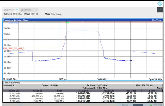
Band2-1.4MHz-QPSK-19193-6RB#0
