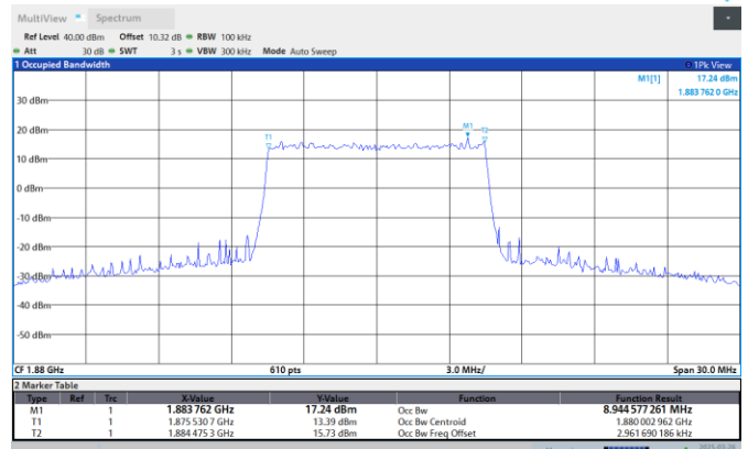
Band2-10MHz-64QAM-18650-50RB#0
