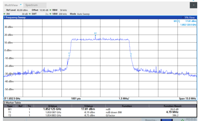
Band2-5MHz-16QAM-19175-25RB#0
