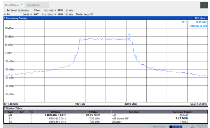
Band2-1.4MHz-16QAM-18607-6RB#0
