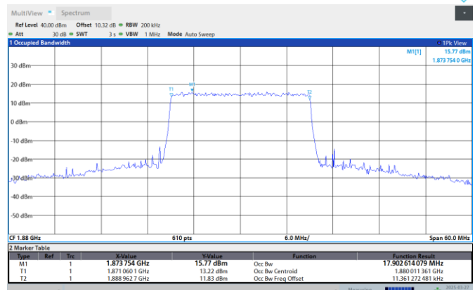
Band2-20MHz-64QAM-18700-100RB#0
