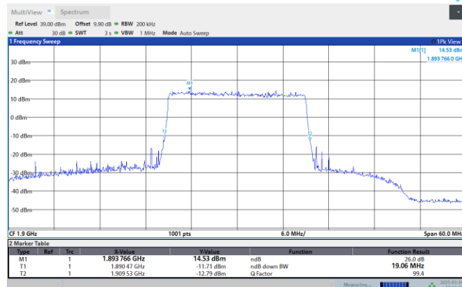
Band2-20MHz-64QAM-19100-100RB#0
