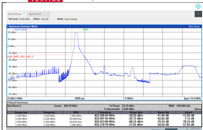
Band5-5MHz-QPSK-20625-1RB#24
