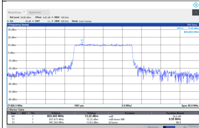
Band5-10MHz-64QAM-20525-50RB#0
