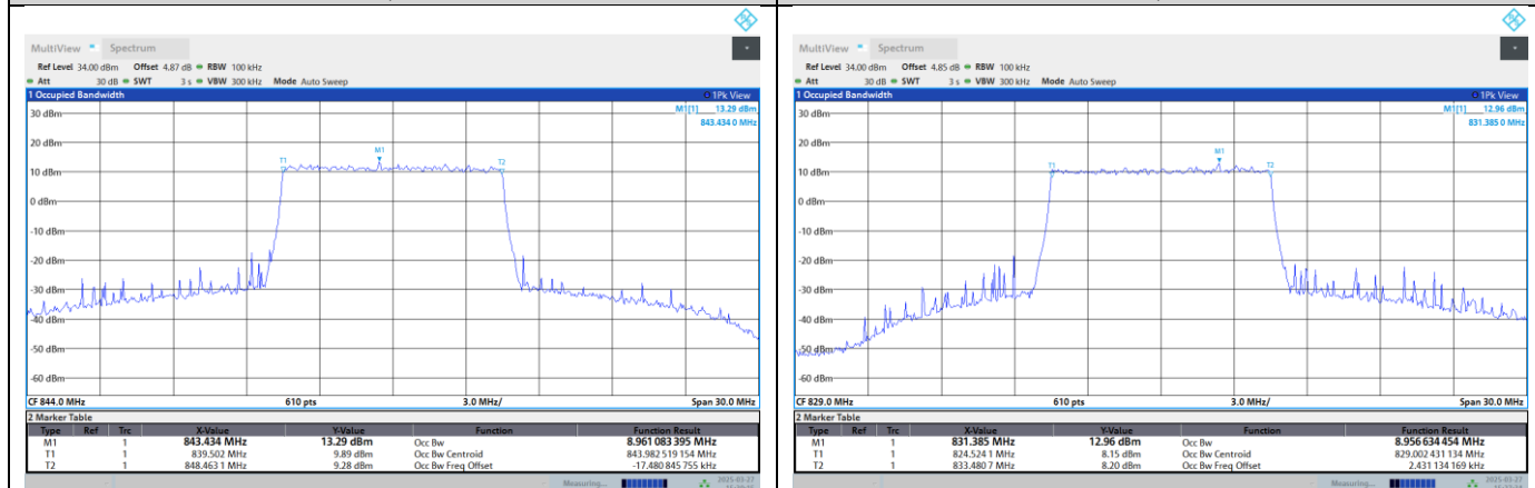
Band5-10MHz-64QAM-20525-50RB#0
