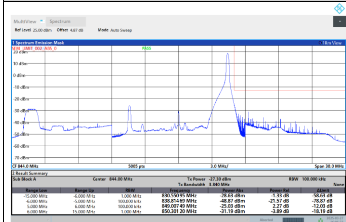
Band5-10MHz-64QAM-20600-1RB#49
