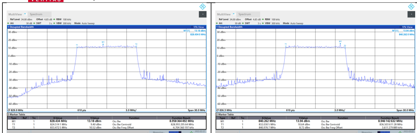
Band5-10MHz-16QAM-20600-50RB#0
