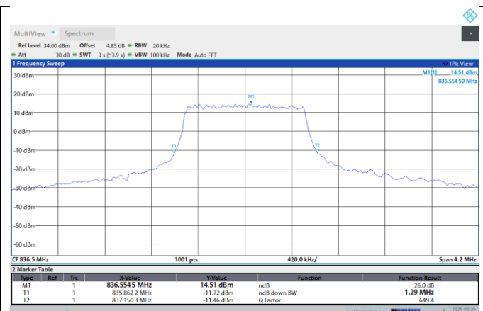
Band5-1.4MHz-16QAM-20407-6RB#0
