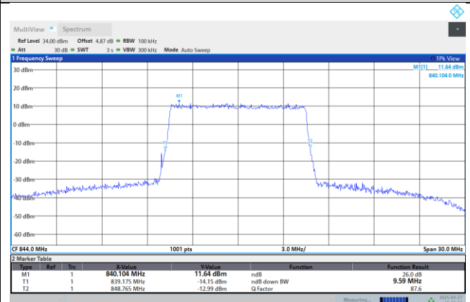
Band5-10MHz-64QAM-20600-50RB#0
