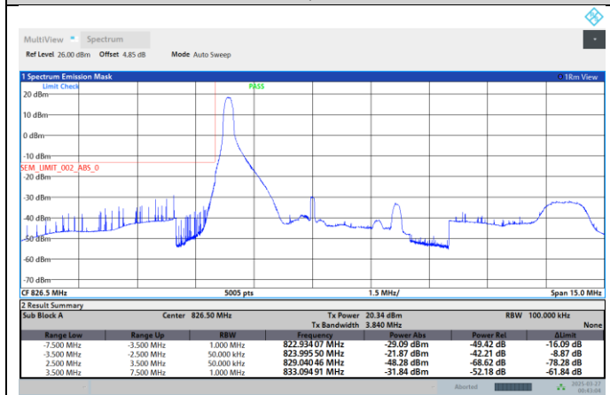
Band5-5MHz-64QAM-20625-1RB#24
