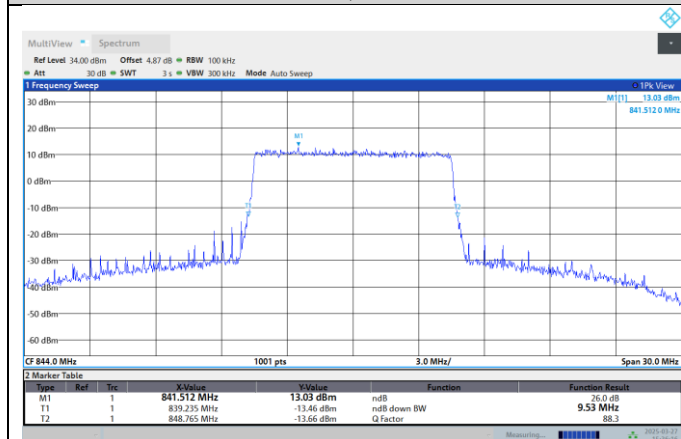
Band5-10MHz-64QAM-20525-50RB#0
