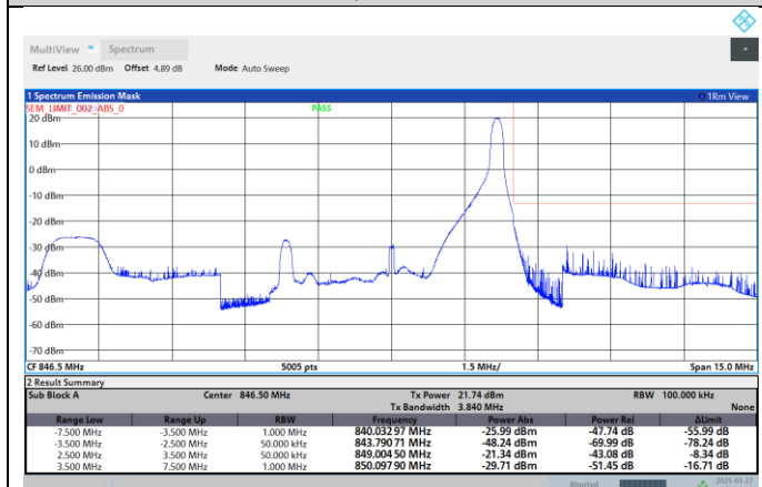
Band5-5MHz-16QAM-20425-1RB#0
