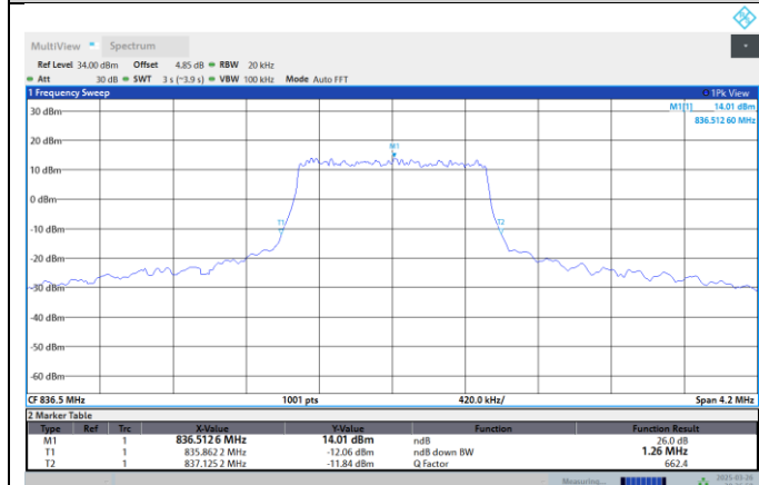
Band5-1.4MHz-64QAM-20407-6RB#0
