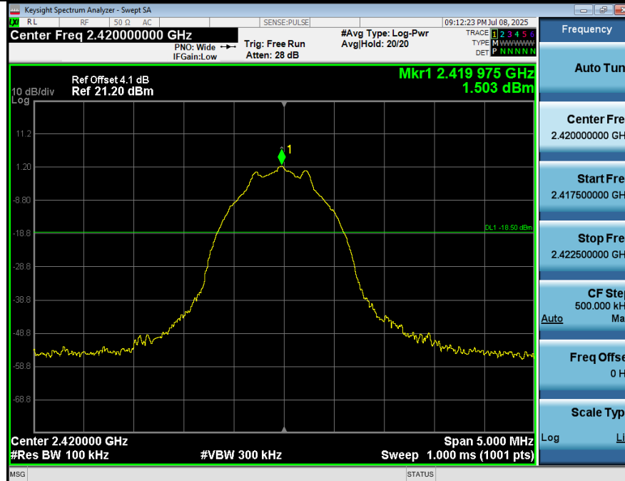
2 Spurious_Emission_NVNT_ANT1_1Mbps_2420
