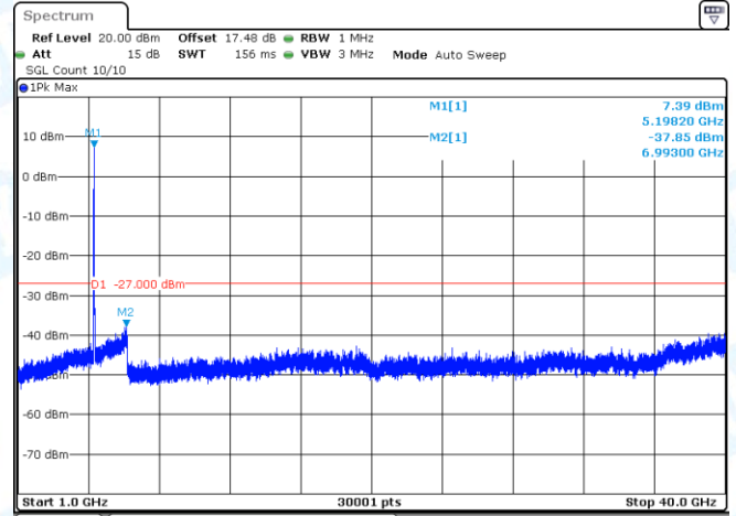
11AX40MIMO-Ant2-5190-1000~40000-PASS
