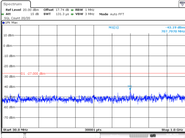
11AX20MIMO-Ant1-5825-30~1000-PASS
