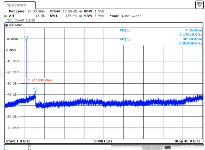
11AX20MIMO-Ant2-5180-1000~40000-PASS
