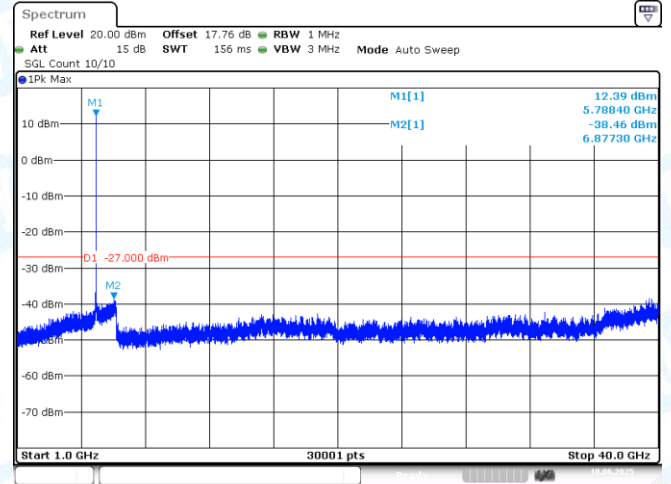
11A-CDD-Ant2-5785-1000~40000-PASS
