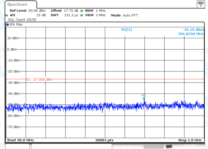
11AC40MIMO-Ant2-5755-30~1000-PASS
