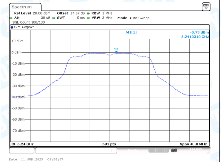
11A-CDD-Ant2-5240-PASS
