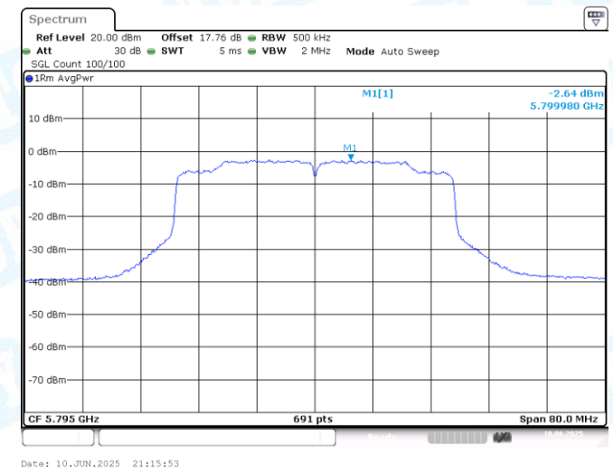
11AX40MIMO-Ant2-5795-PASS
