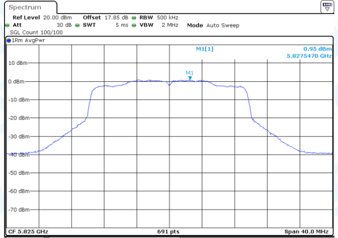
11AX20MIMO-Ant2-5825-PASS
