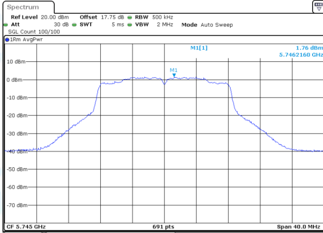
11A-CDD-Ant1-5745-PASS
