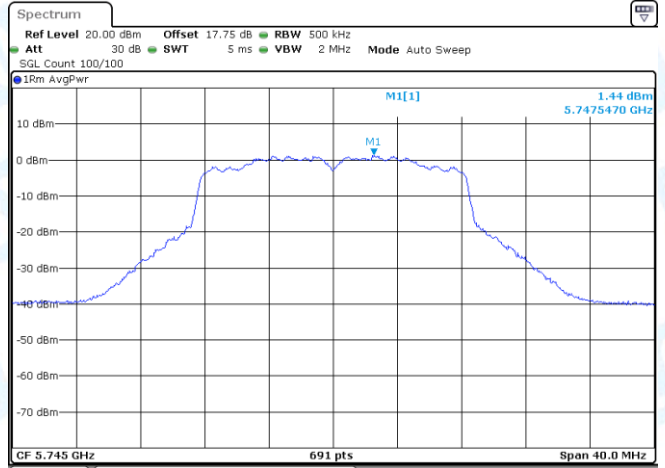
11A-CDD-Ant2-5745-PASS
