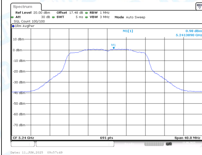
11A-CDD-Ant1-5240-PASS
