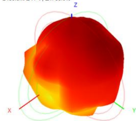
2450.0MHz H+V, Eff: 55.8%
