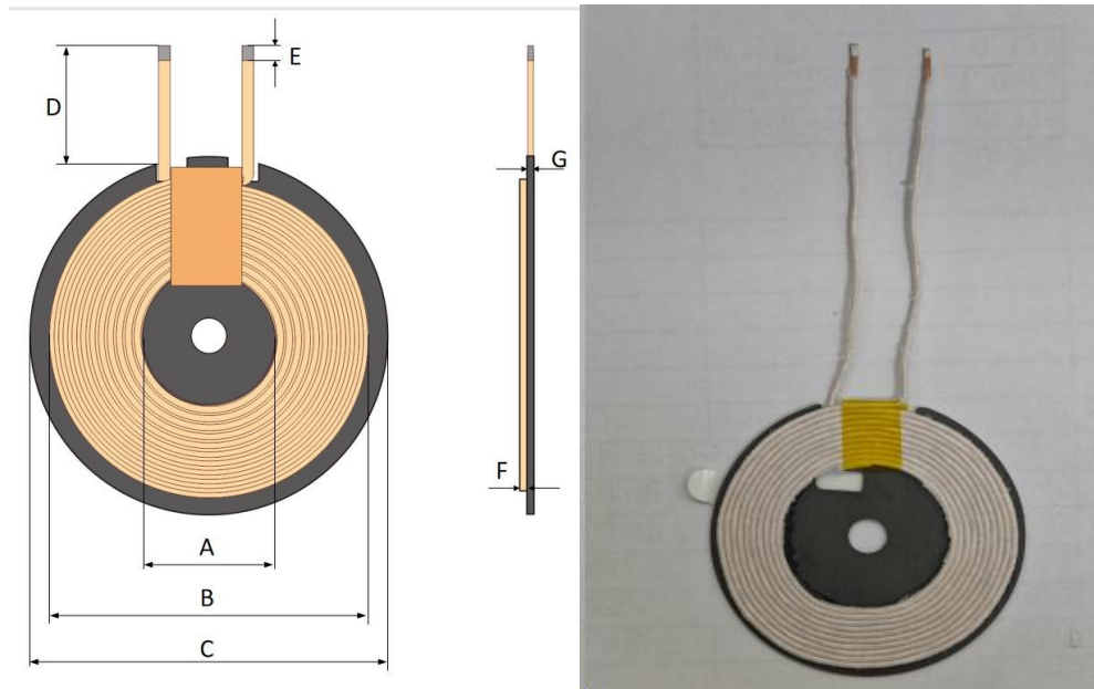
Model drawing
