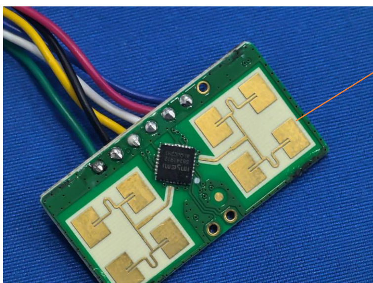
Radar ANT
