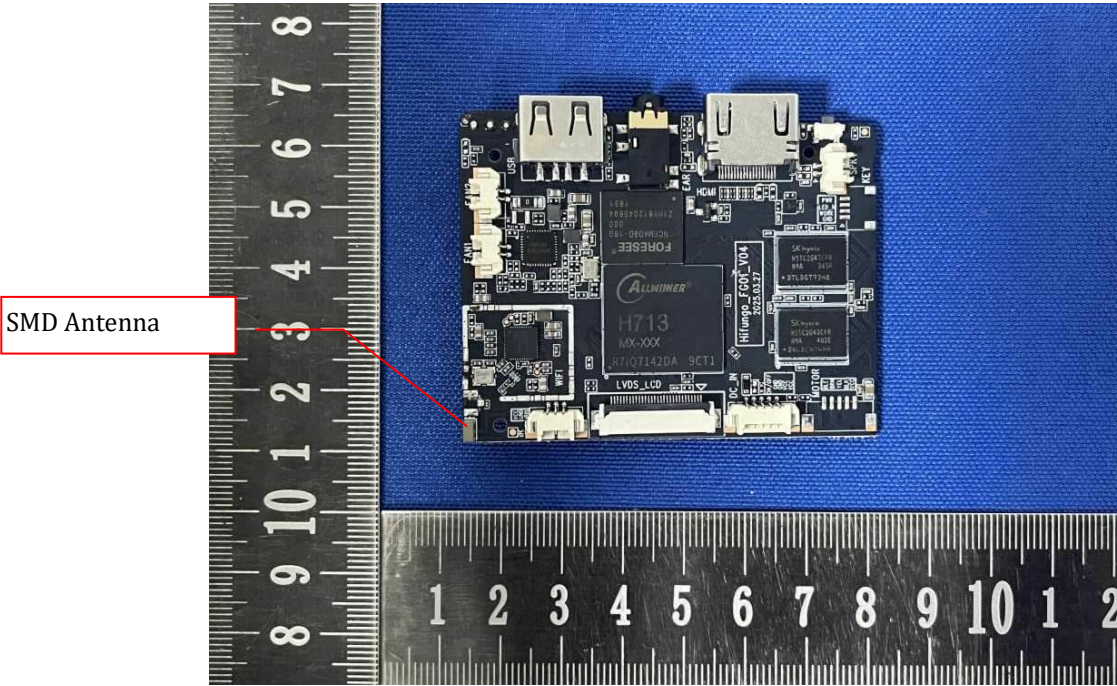
EUT Internal View 3
