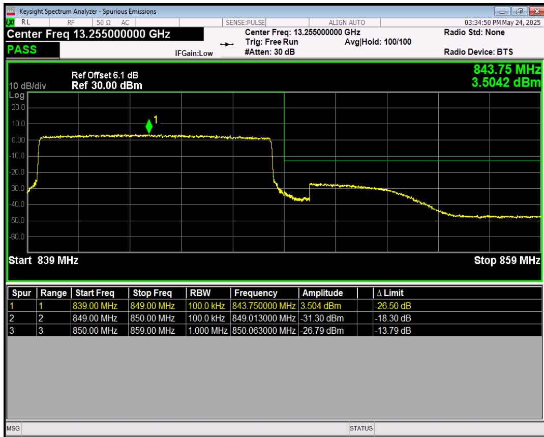
Band5 64QAM BW=10MHz Channel=20600 RB Size=1 Position=#0
