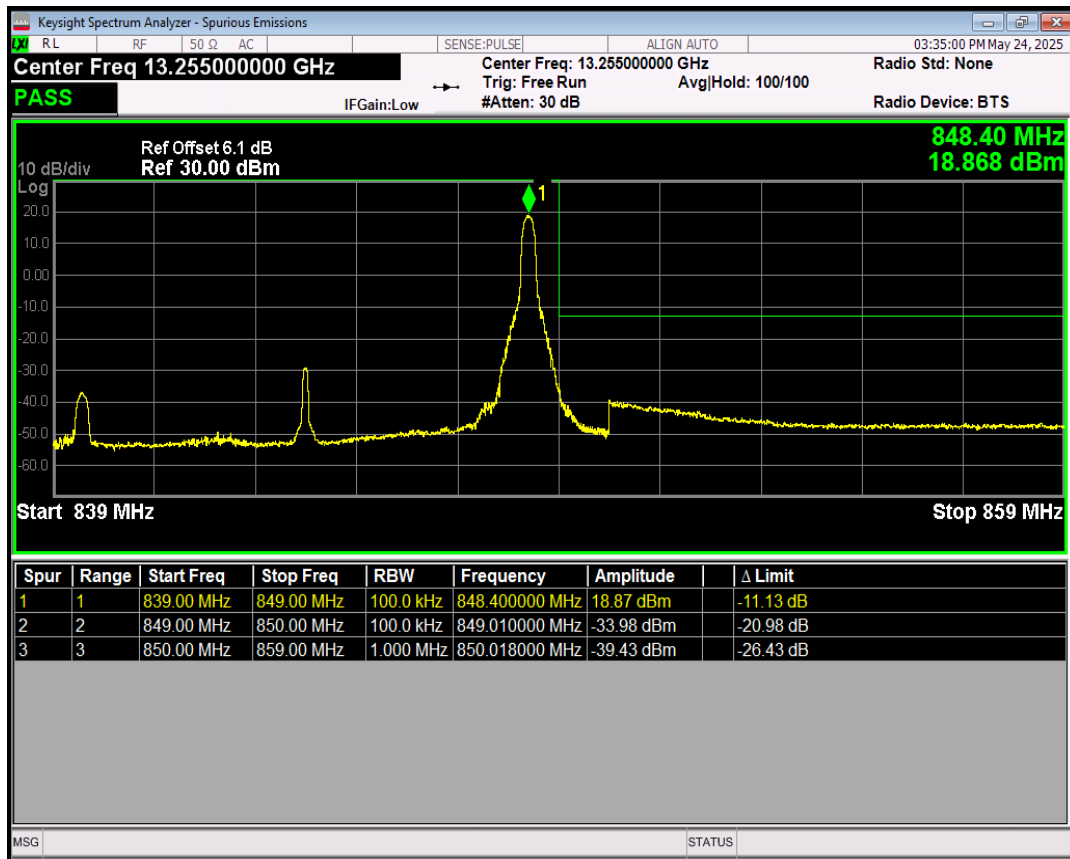
Band5 64QAM BW=10MHz Channel=20600 RB Size=50 Position=#0
