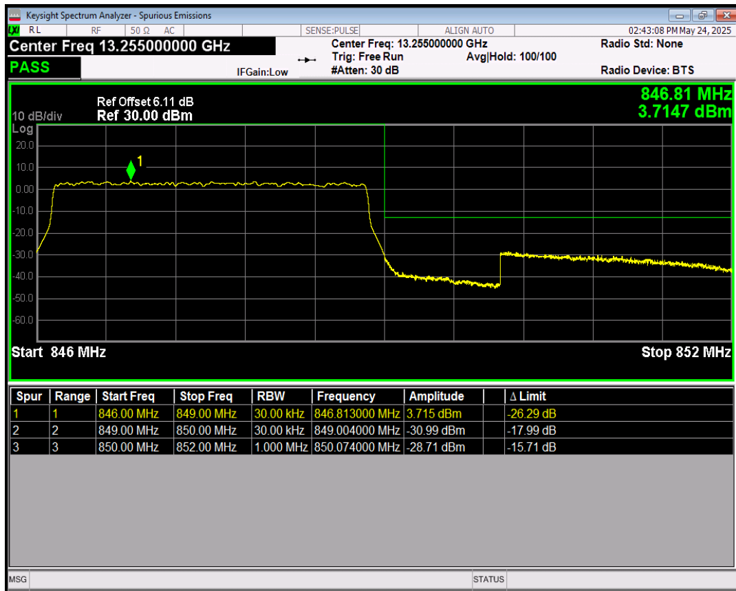
Band5 64QAM BW=3MHz Channel=20635 RB Size=1 Position=#0
