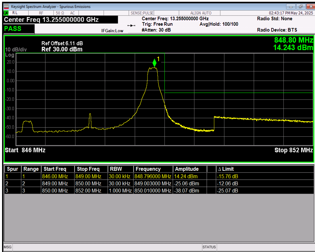
Band5 64QAM BW=3MHz Channel=20635 RB Size=15 Position=#0
