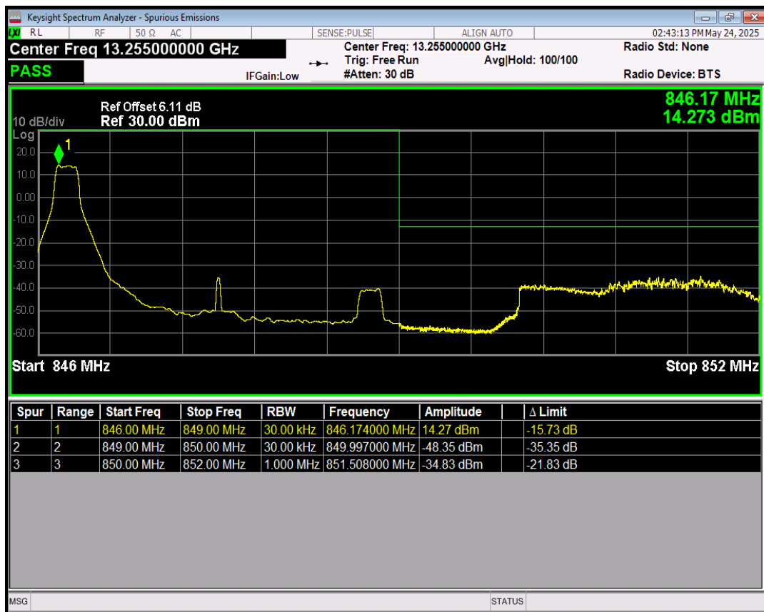
Band5 64QAM BW=3MHz Channel=20635 RB Size=1 Position=#Max
