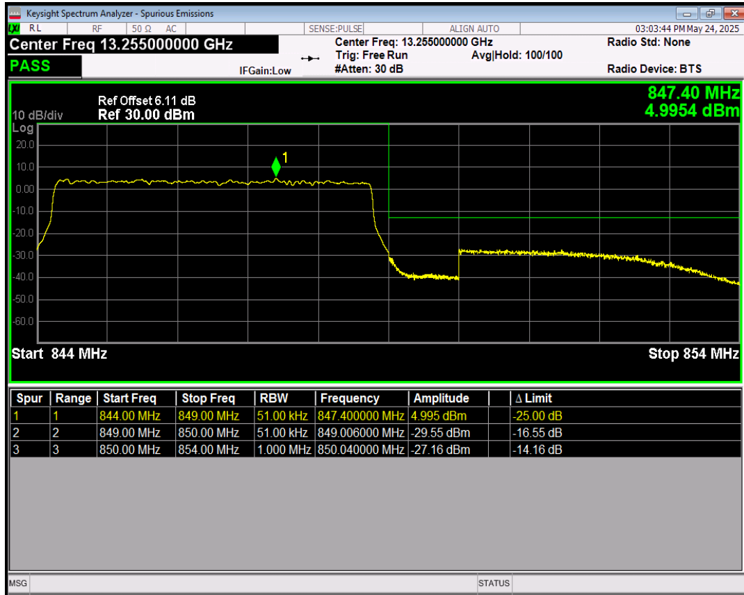
Band5 64QAM BW=5MHz Channel=20625 RB Size=1 Position=#0
