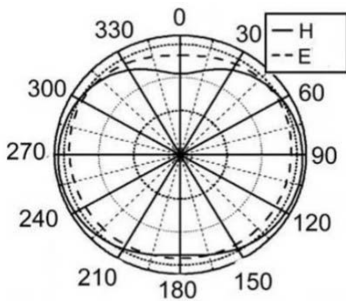
27.145 MHz radiation pattern
