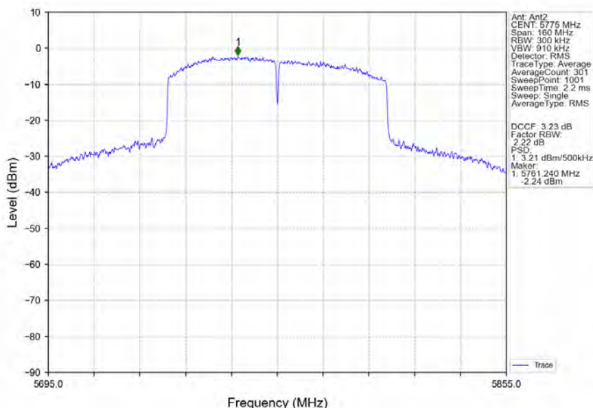
802.11ac(VHT80)_MCH_5775MHz_Ant2_NTNV
