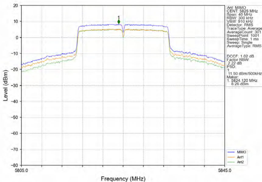
802.11ac(VHT20)_HCH_5825MHz_MIMO_NTNV
