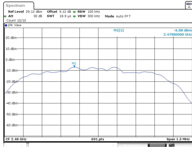
3DH5_Ant1_2480_0~Reference
