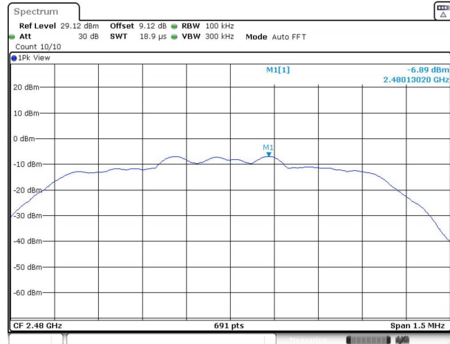
2DH5_Ant1_2480_0~Reference
