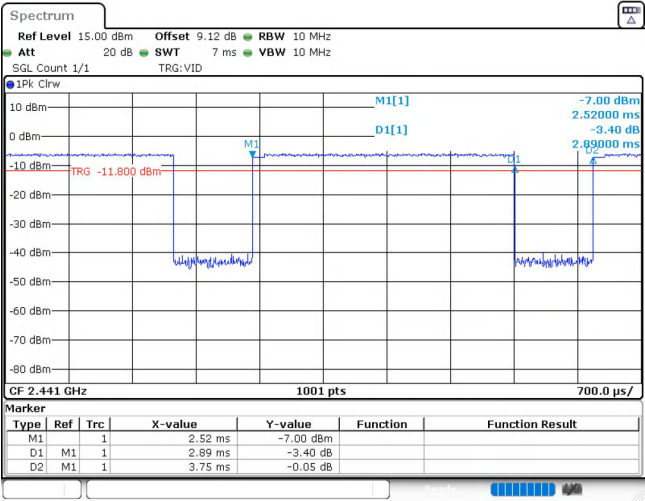
2DH5_Ant1_2441
