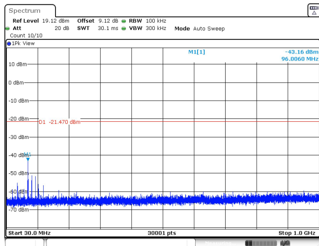
BLE_1M_Ant1_2480_0~Reference
