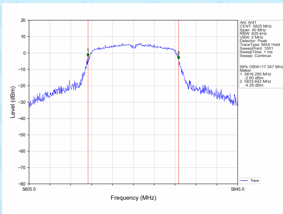
802.11a_HCH_5825MHz_Ant1_NTNV
