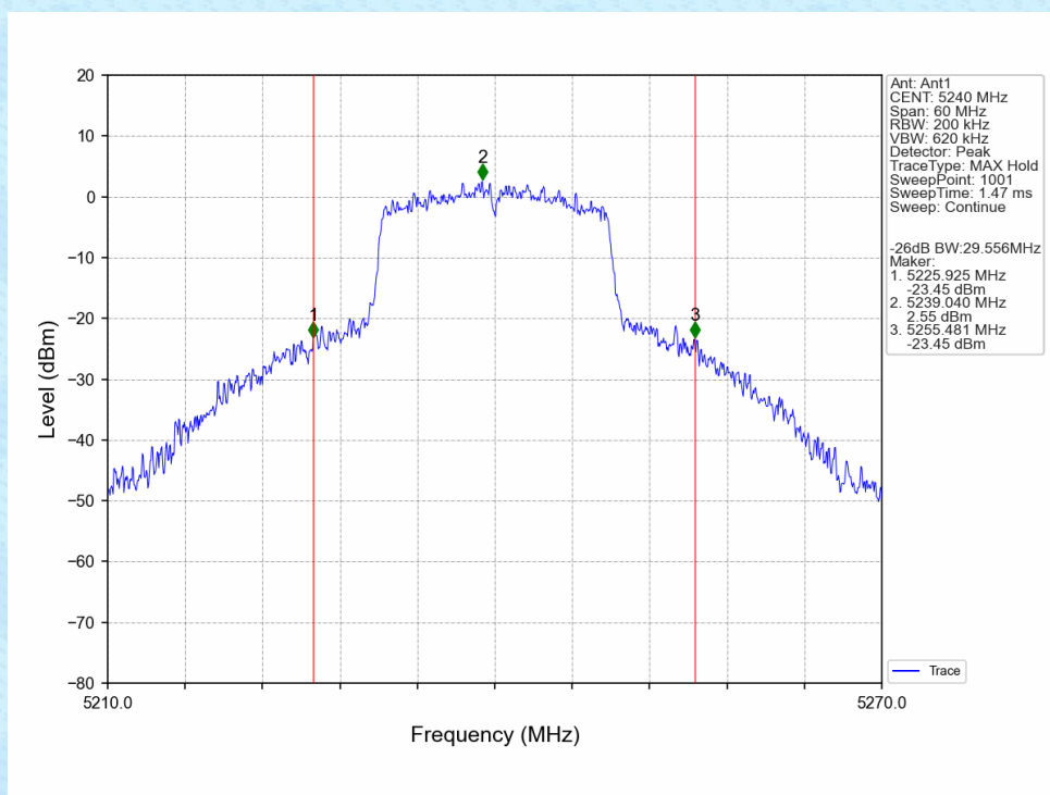
802.11n(HT20)_HCH_5240MHz_Ant1_NTNV
