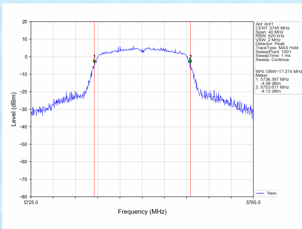
802.11a_LCH_5745MHz_Ant1_NTNV
