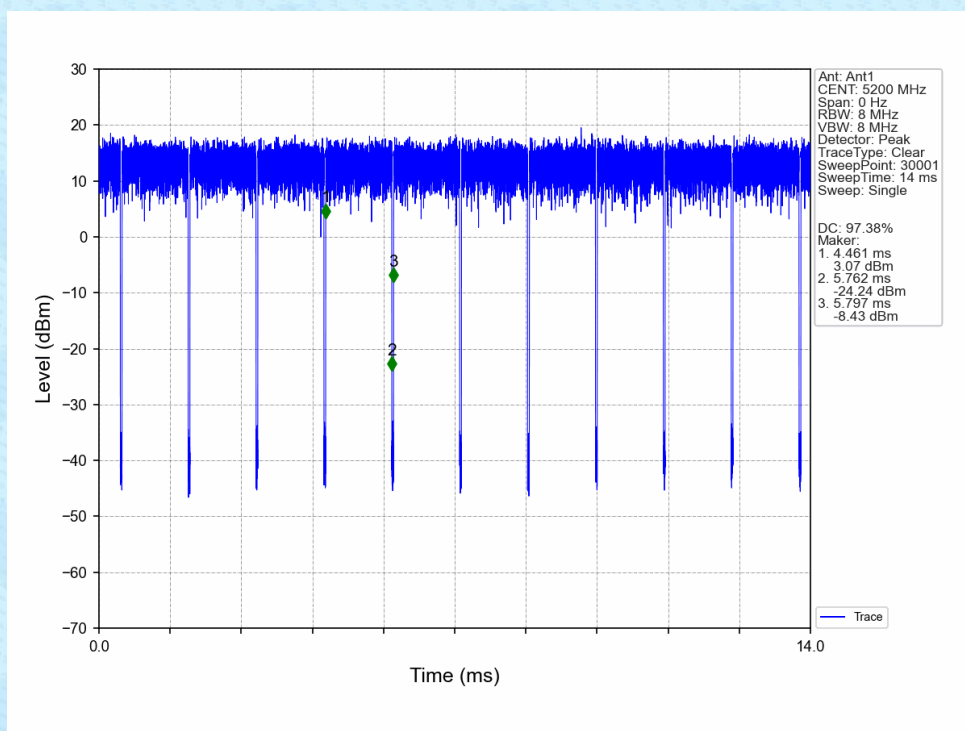
802.11n(HT20)_MCH_5200MHz_Ant1_NTNV
