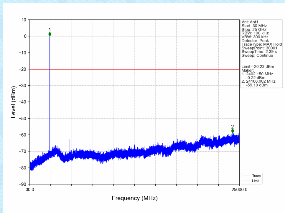
GFSK_DH5_LCH_2402MHz_Ant1_NTNV
