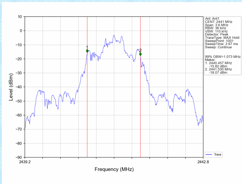
8DPSK_3DH5_MCH_2441MHz_Ant1_NTNV
