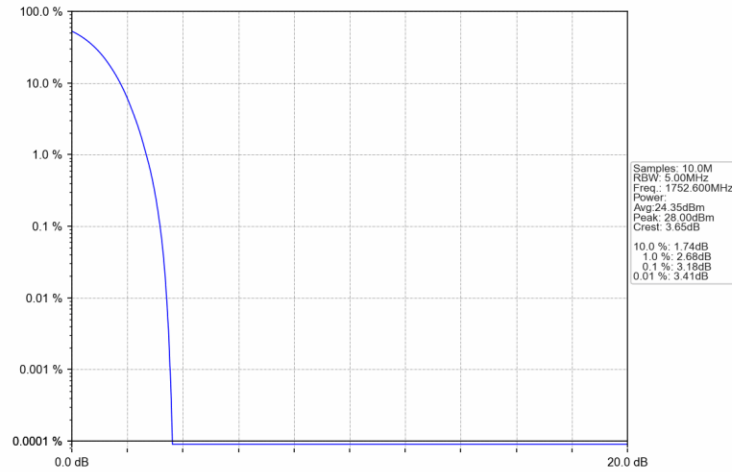
Band4_RMC_HCH_1752.6MHz_12.2kbps RMC_NTNV
