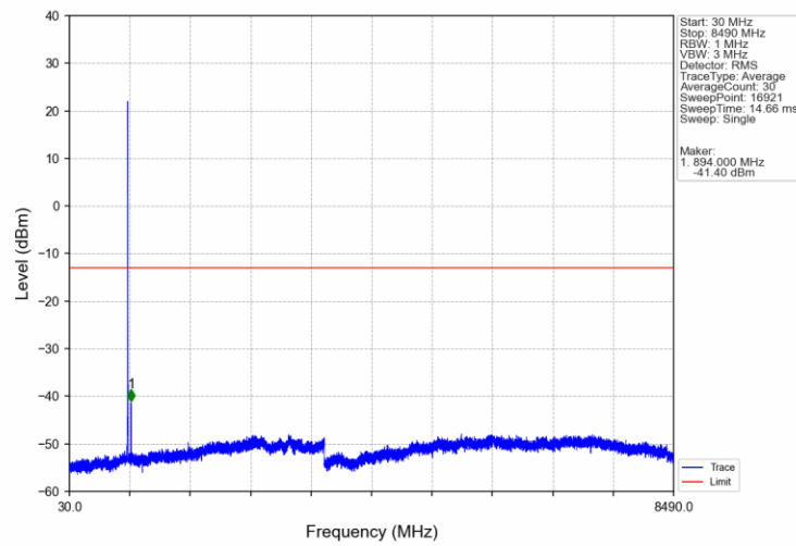
Band5_3MHz_16QAM_HCH_847.5MHz_RB_1_0_NTNV
