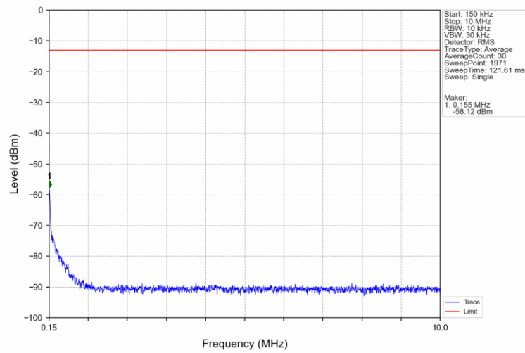
Band5_5MHz_16QAM_MCH_836.5MHz_RB_1_0_NTNV
