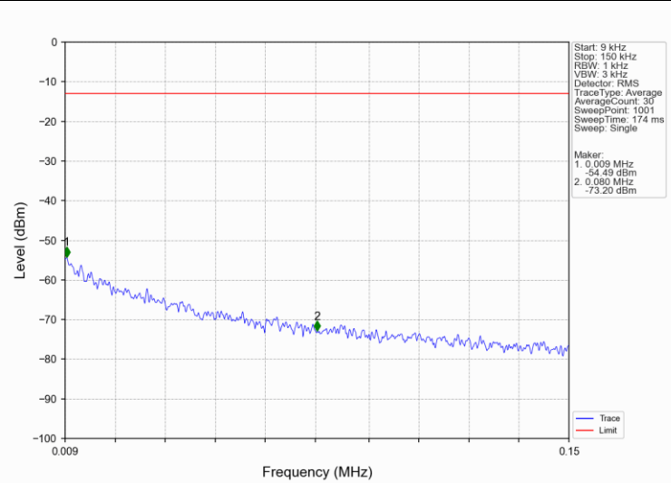
Band5_3MHz_16QAM_HCH_847.5MHz_RB_1_0_NTNV
