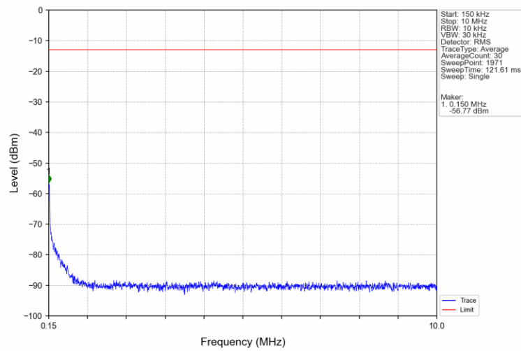
Band5_5MHz_QPSK_HCH_846.5MHz_RB_1_0_NTNV
