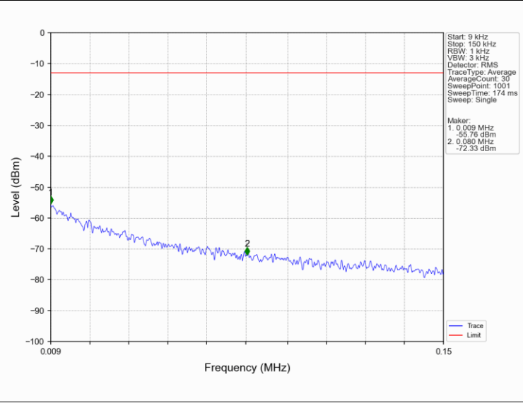
Band5 1.4MHz 16QAM MCH 836.5MHz RB 1 0 NTNV
