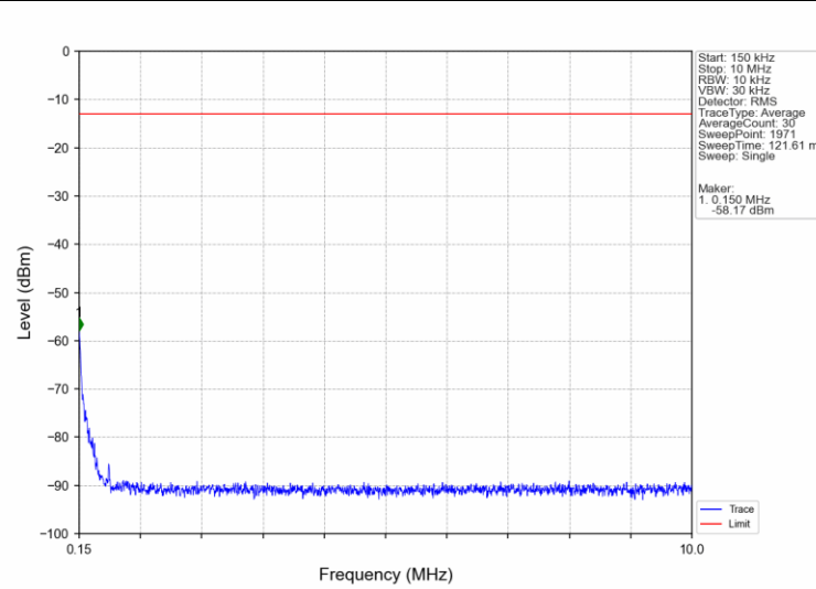
Band5 1.4MHz 16QAM MCH 836.5MHz RB 1 0 NTNV
