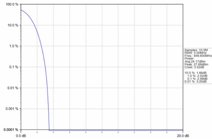
Band5_RMC_HCH_846.6MHz_12.2kbps RMC_NTNV
