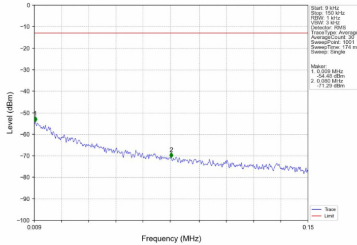
Band2_RMC_LCH_1852.4MHz_12.2kbps RMC_NTNV
