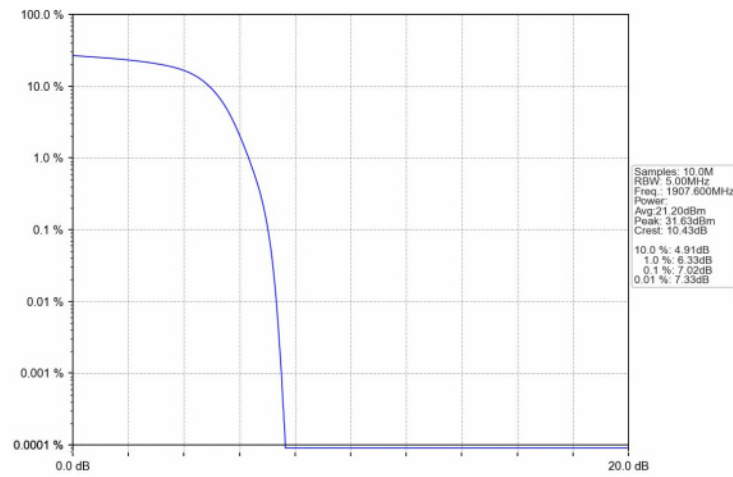
Band2_HSUPA_HCH_1907.6MHz_Subtest 1_NTNV
