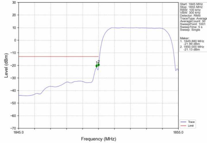
Band2_RMC_LCH_1852.4MHz_12.2kbps RMC_NTNV
