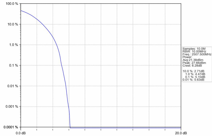
Band7_15MHz_QPSK_LCH_2507.5MHz_RB_75_0_NTNV
