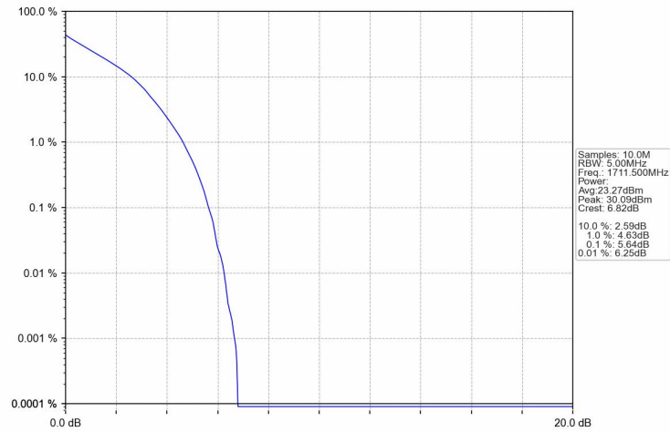
Band4_3MHz_QPSK_LCH_1711.5MHz_RB_15_0_NTNV
