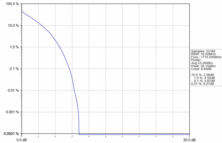
Band4_10MHz_QPSK_LCH_1715MHz_RB_50_0_NTNV
