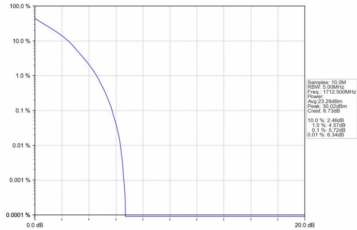
Band4_5MHz_QPSK_LCH_1712.5MHz_RB_25_0_NTNV
