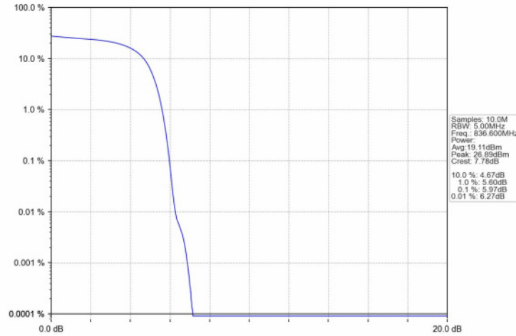
Band5_HSDPA_MCH_836.6MHz_Subtest 1_NTNV
