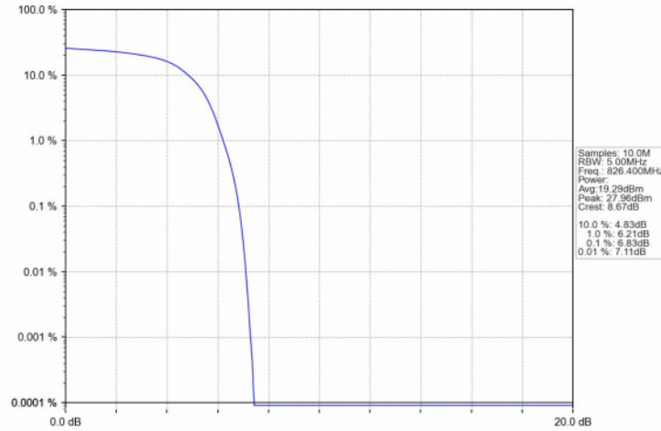
Band5_HSUPA_LCH_826.4MHz_Subtest 1_NTNV
