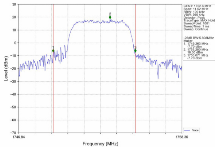
Band4_HSDPA_HCH_1752.6MHz_Subtest 1_NTNV
