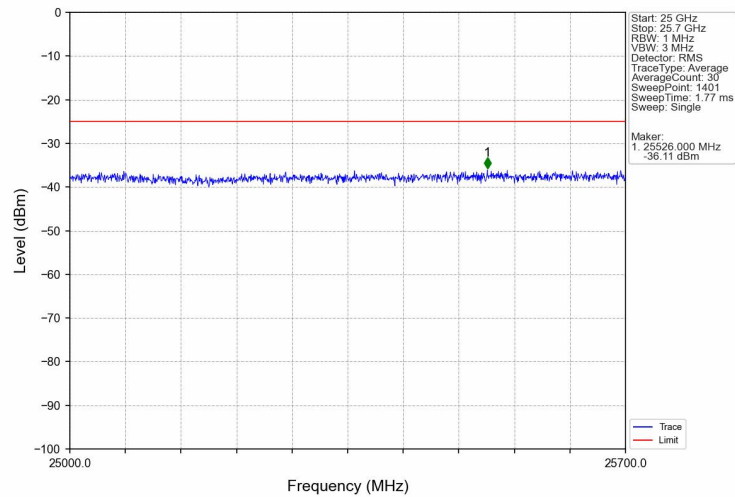
Band7_5MHz_16QAM_MCH_2535MHz_RB_1_0_NTNV
