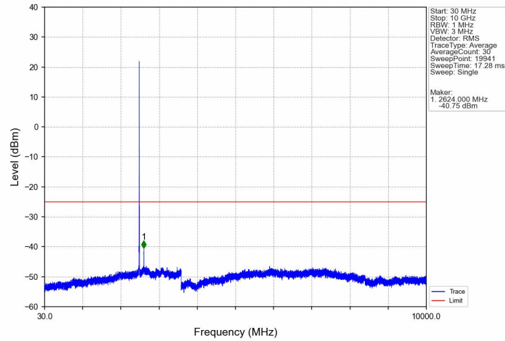
Band7_5MHz_16QAM_LCH_2502.5MHz_RB_1_0_NTNV
