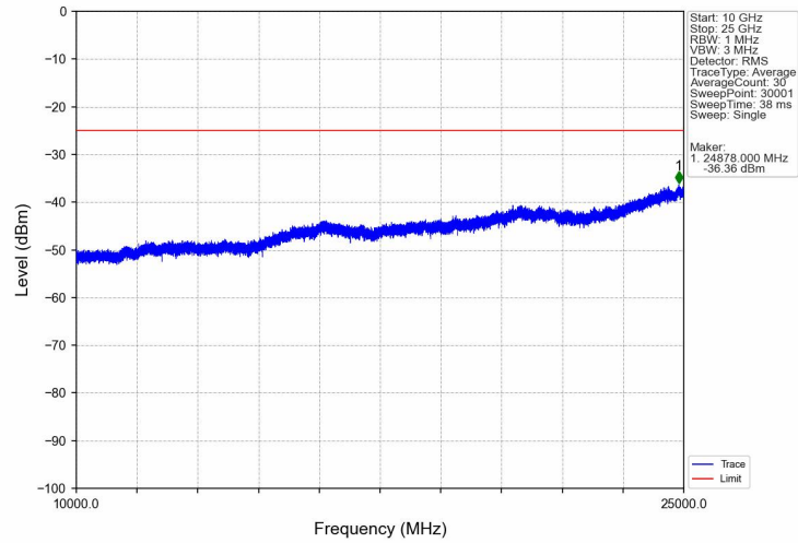
Band7_5MHz_16QAM_HCH_2567.5MHz_RB_1_0_NTNV
