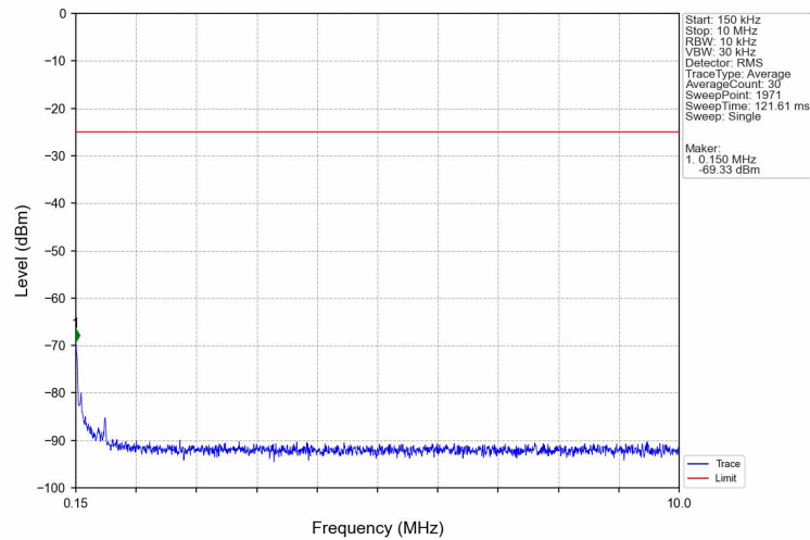
Band7_5MHz_16QAM_MCH_2535MHz_RB_1_0_NTNV
