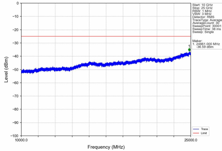
Band7_5MHz_16QAM_MCH_2535MHz_RB_1_0_NTNV
