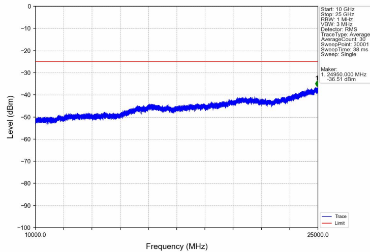
Band7_5MHz_16QAM_LCH_2502.5MHz_RB_1_0_NTNV
