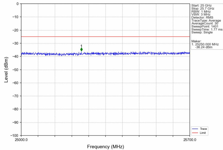
Band7_5MHz_16QAM_HCH_2567.5MHz_RB_1_0_NTNV
