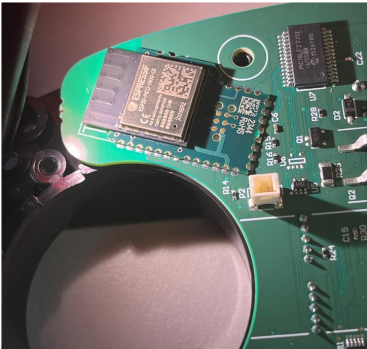
Figure 3 Espressif Original FCCID Location
