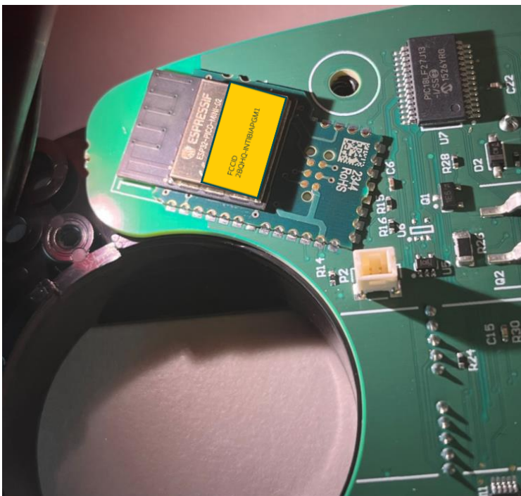
Figure 4 Coloplast FCCID Label Location (simulated)
