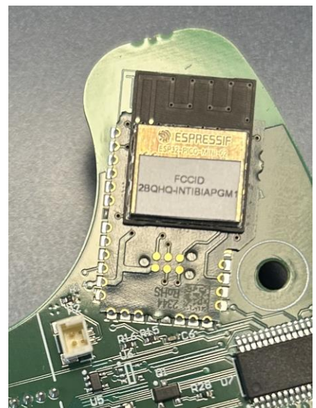
Figure 5 Example Coloplast FCCID Label Location
