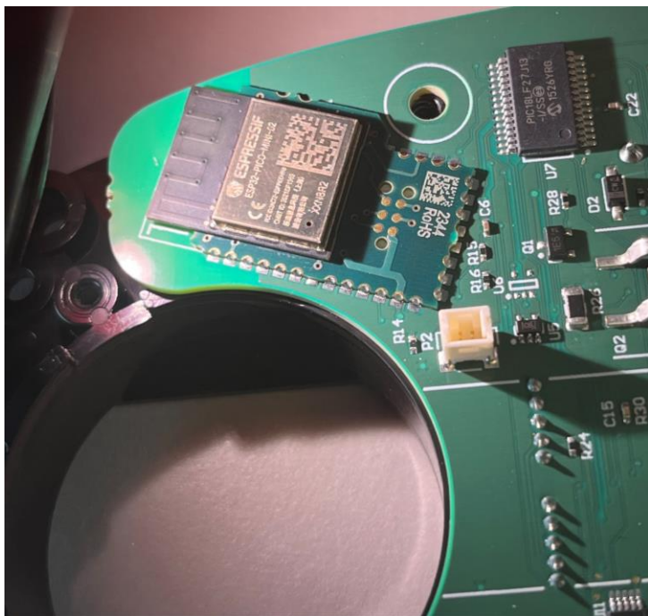
Figure 1 Espressif ESP32-Pico-Mini-02 Module on Coloplast Intibia Wand Model CP-IN200
