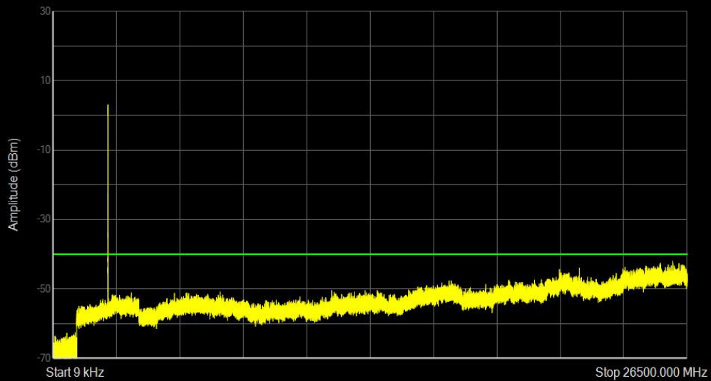
Band40(2305-2315) QPSK BW=5MHz Channel=38750 RB Size=25 Position=#0
