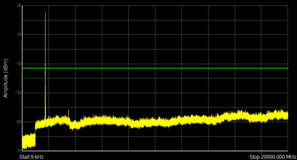
Band4 16QAM BW=10MHz Channel=20350 RB Size=1 Position=#Mid
