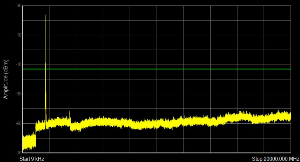
Band4 16QAM BW=20MHz Channel=20300 RB Size=1 Position=#Mid
