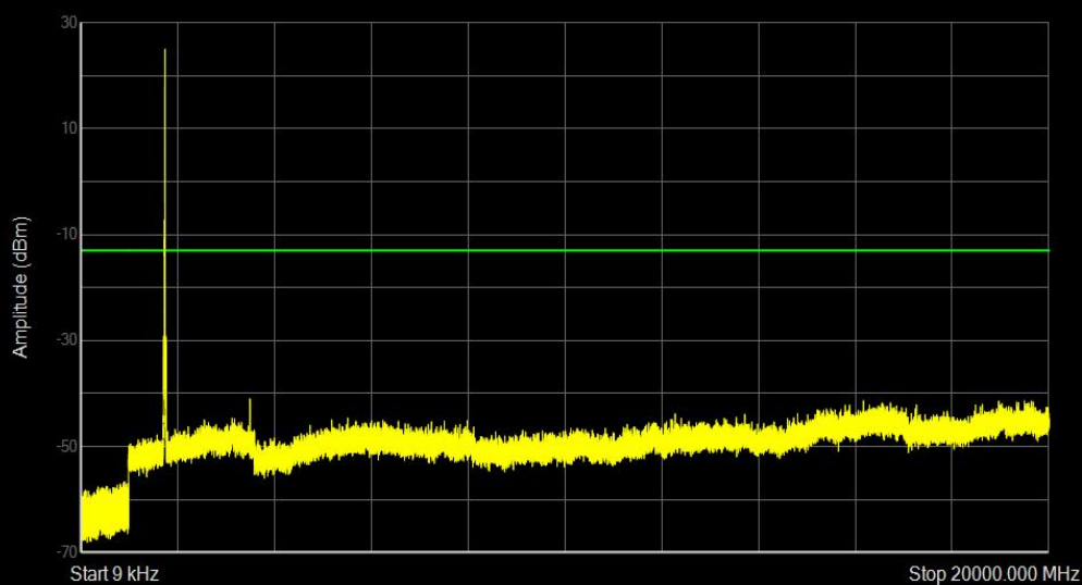
Band4 16QAM BW=15MHz Channel=20325 RB Size=1 Position=#Mid
