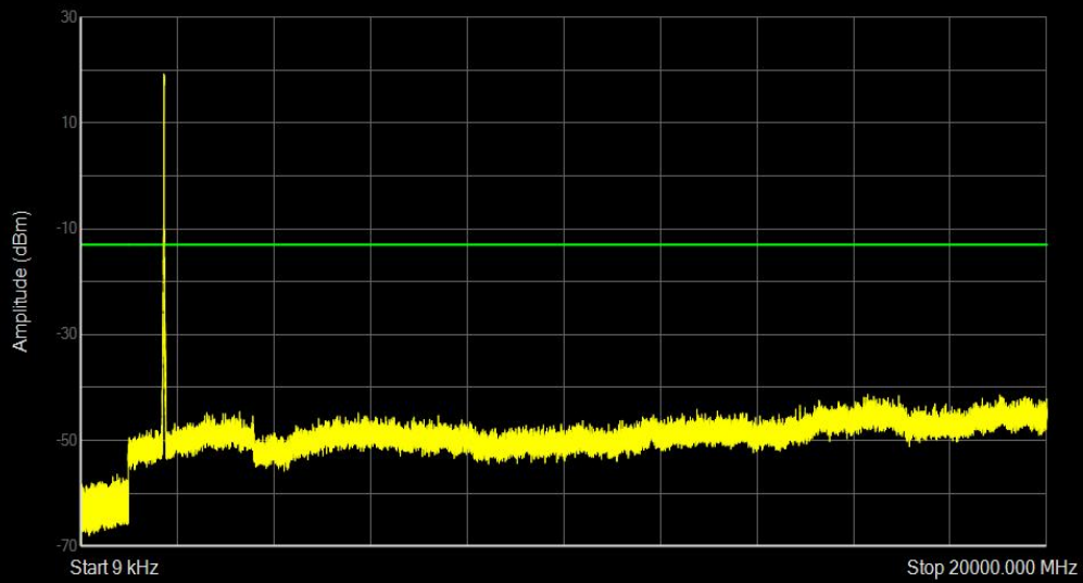
Band4 QPSK BW=20MHz Channel=20300 RB Size=1 Position=#Max
