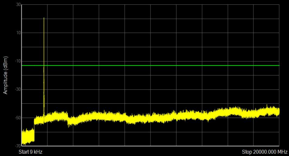
Band4 16QAM BW=10MHz Channel=20350 RB Size=25 Position=#0
