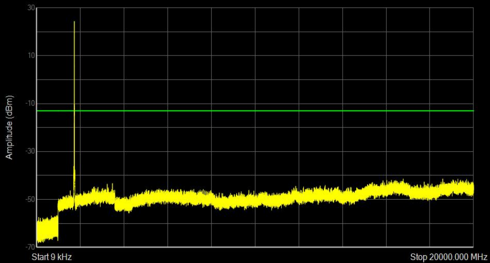
Band4 QPSK BW=20MHz Channel=20300 RB Size=1 Position=#0
