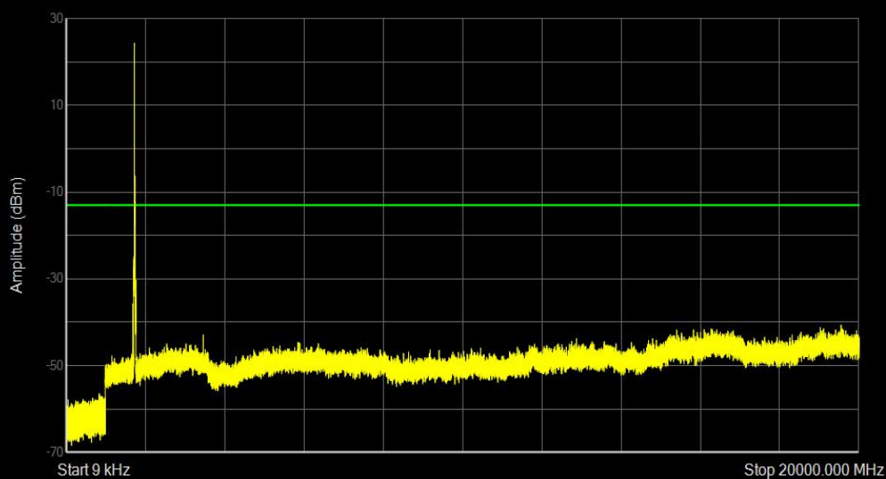
Band4 QPSK BW=20MHz Channel=20300 RB Size=50 Position=#Max
