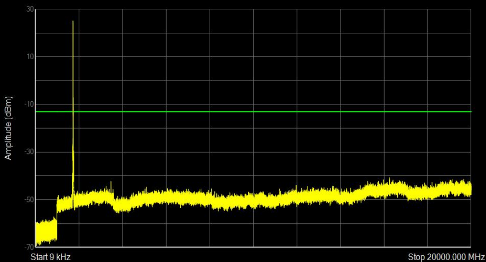
Band4 QPSK BW=15MHz Channel=20325 RB Size=36 Position=#Max
