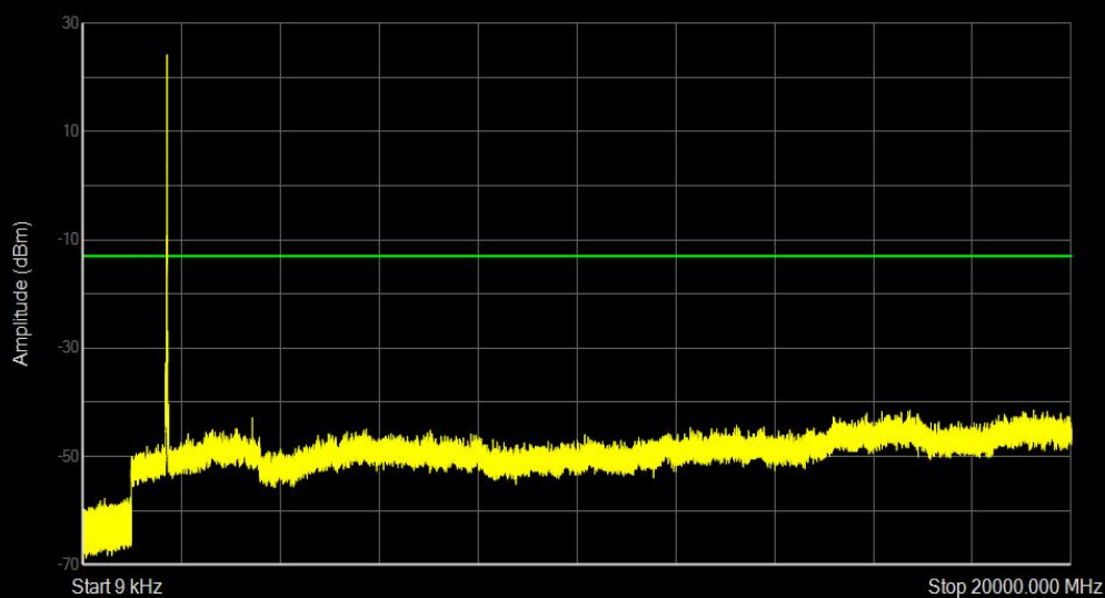
Band4 16QAM BW=15MHz Channel=20025 RB Size=1 Position=#Mid
