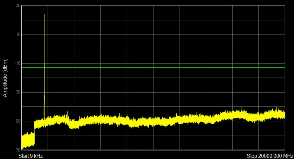
Band4 QPSK BW=10MHz Channel=20350 RB Size=25 Position=#Max
