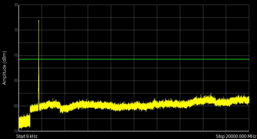
Band4 16QAM BW=20MHz Channel=20300 RB Size=50 Position=#0
