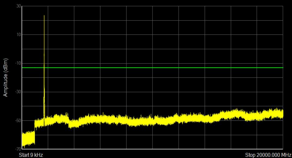
Band4 16QAM BW=20MHz Channel=20050 RB Size=1 Position=#Mid
