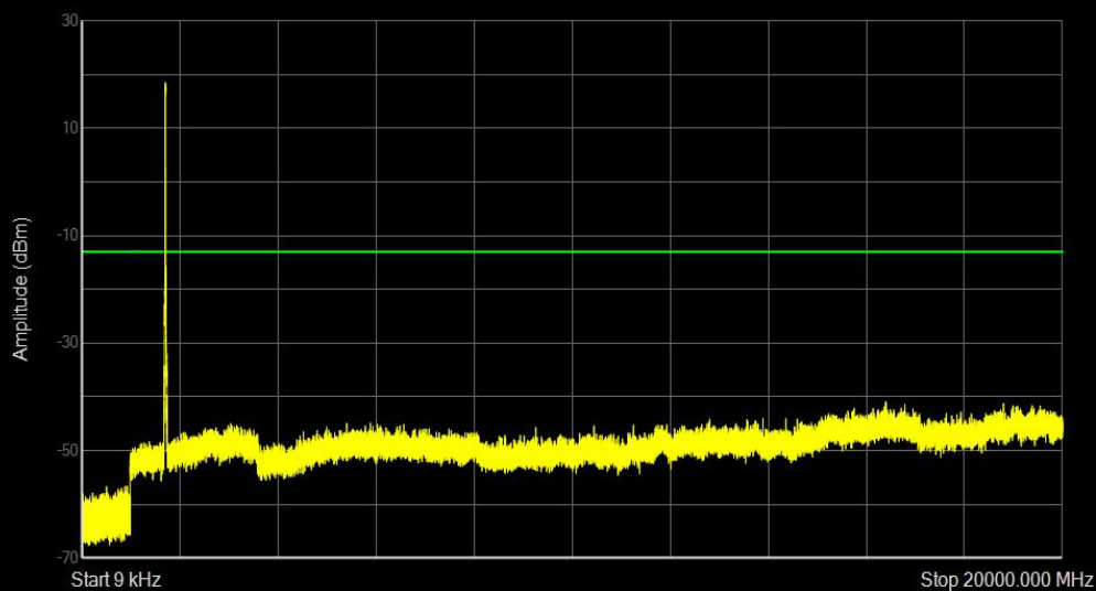
Band4 QPSK BW=20MHz Channel=20050 RB Size=1 Position=#Max
