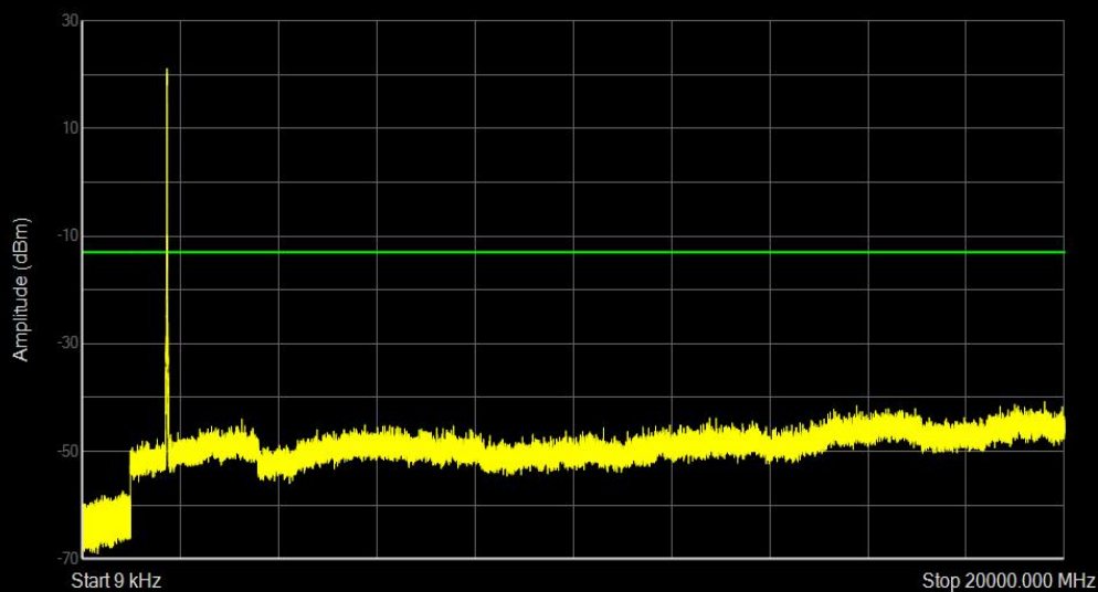
Band4 QPSK BW=15MHz Channel=20325 RB Size=1 Position=#Max
