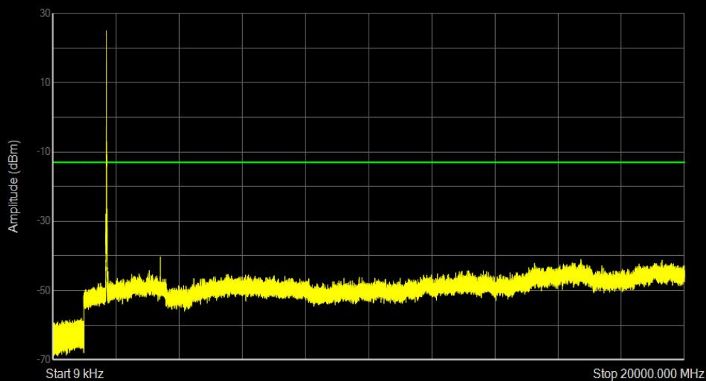
Band4 QPSK BW=15MHz Channel=20025 RB Size=36 Position=#Max
