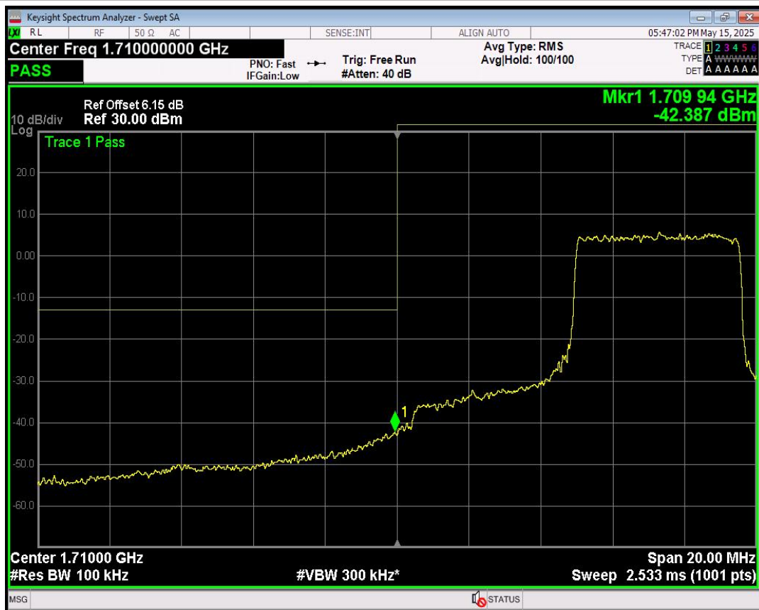
Band4 QPSK BW=10MHz Channel=20000 RB Size=25 Position=#Max
