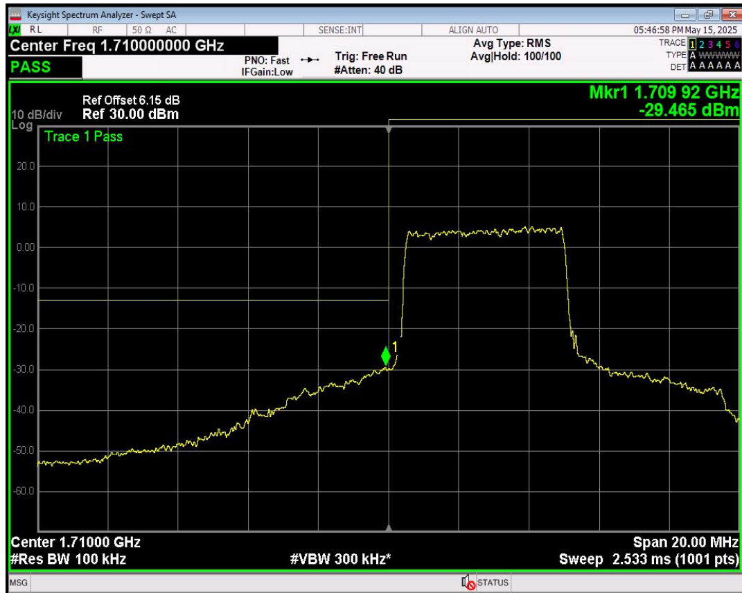
Band4 QPSK BW=10MHz Channel=20000 RB Size=25 Position=#0
