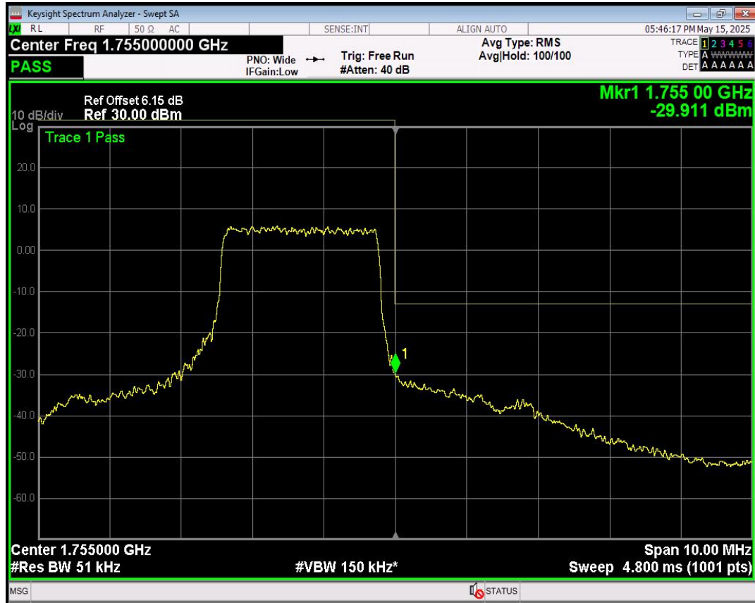
Band4 QPSK BW=5MHz Channel=20375 RB Size=12 Position=#Max
