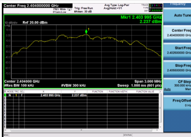
GFSK (BLE 2Mbps) LOW CHANNEL, CARRIER LEVEL
