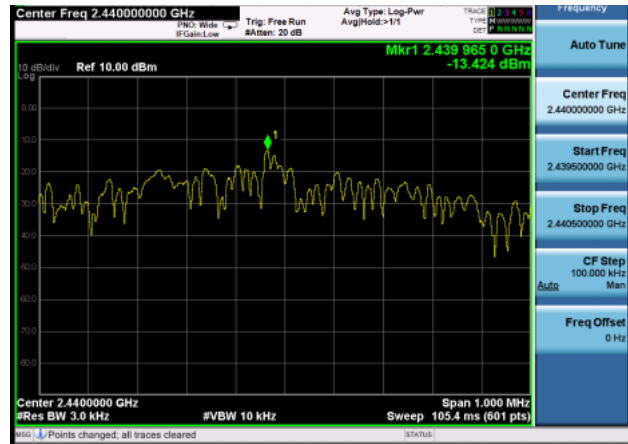
GFSK (BLE 1Mbps) MIDDLE CHANNEL
