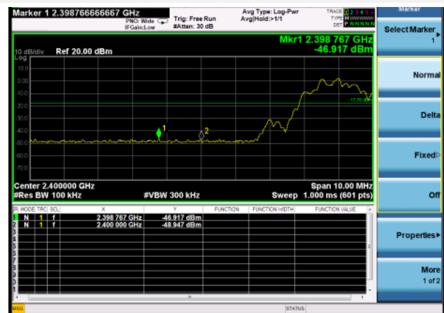
GFSK (BLE 2Mbps) LOW CHANNEL, BAND EDGE
