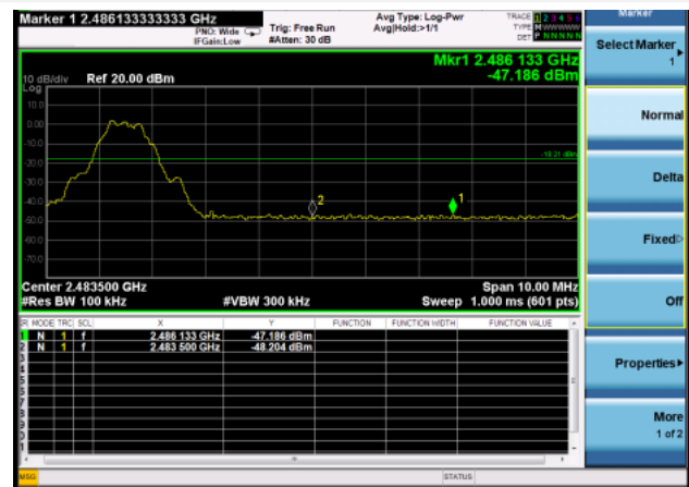
GFSK (BLE 1Mbps) HIGH CHANNEL, BAND EDGE
