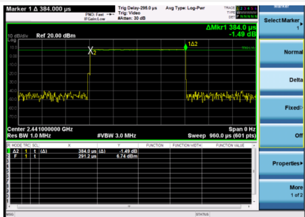
GFSK DH1
