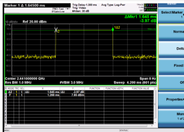
GFSK DH3
