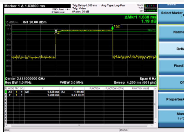
8-DPSK 3DH3
