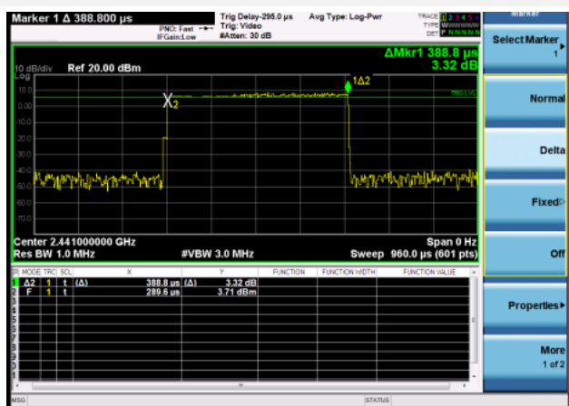
8-DPSK 3DH1
