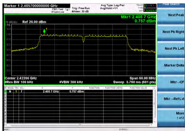
802.11n-40 MHz LOW CHANNEL, CARRIER LEVEL
