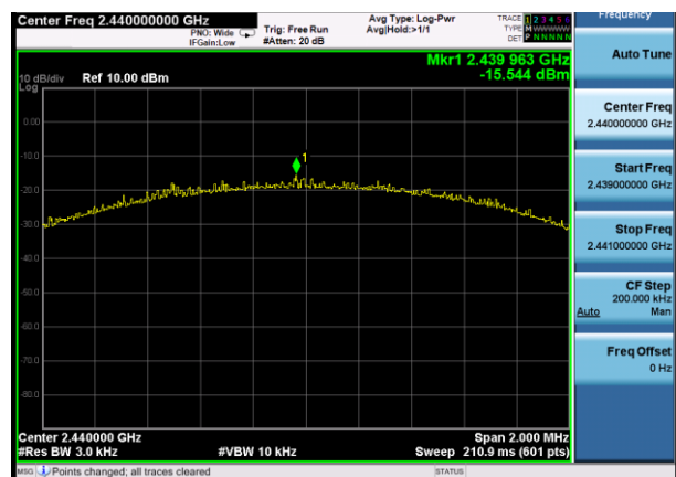
GFSK (BLE 2Mbps) MIDDLE CHANNEL
