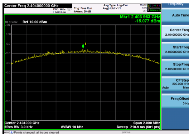
GFSK (BLE 2Mbps) LOW CHANNEL
