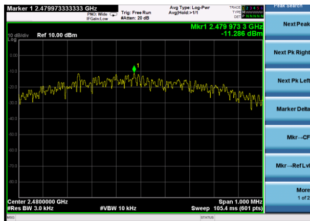
GFSK (BLE 1Mbps) HIGH CHANNEL
