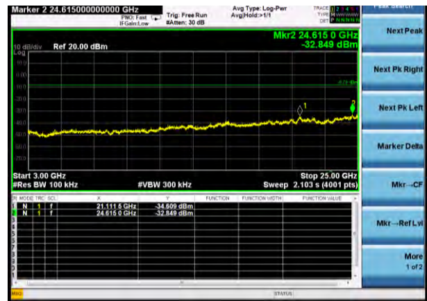
GFSK LOW CHANNEL, SPURIOUS 3 GHz ~ 25 GHz
