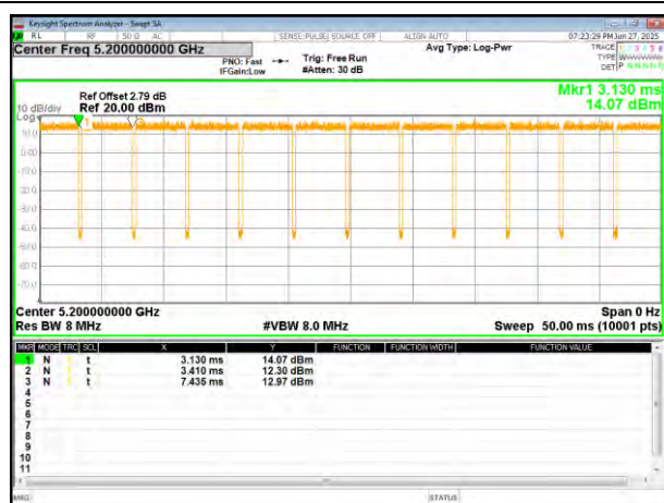
(802.11a) plot
