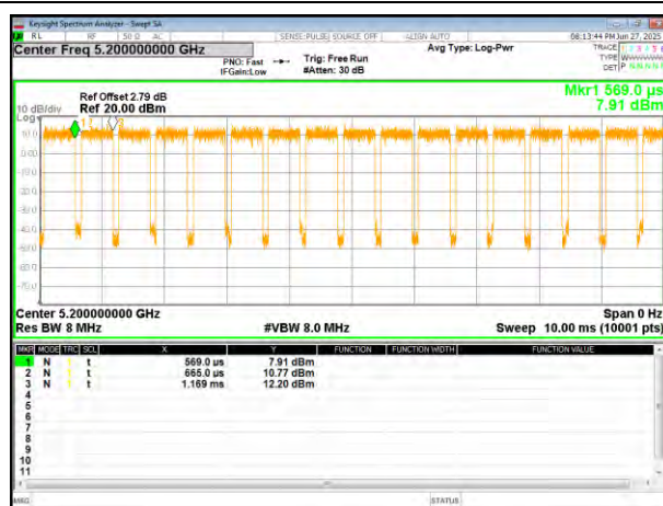
(802.11 n20) plot
