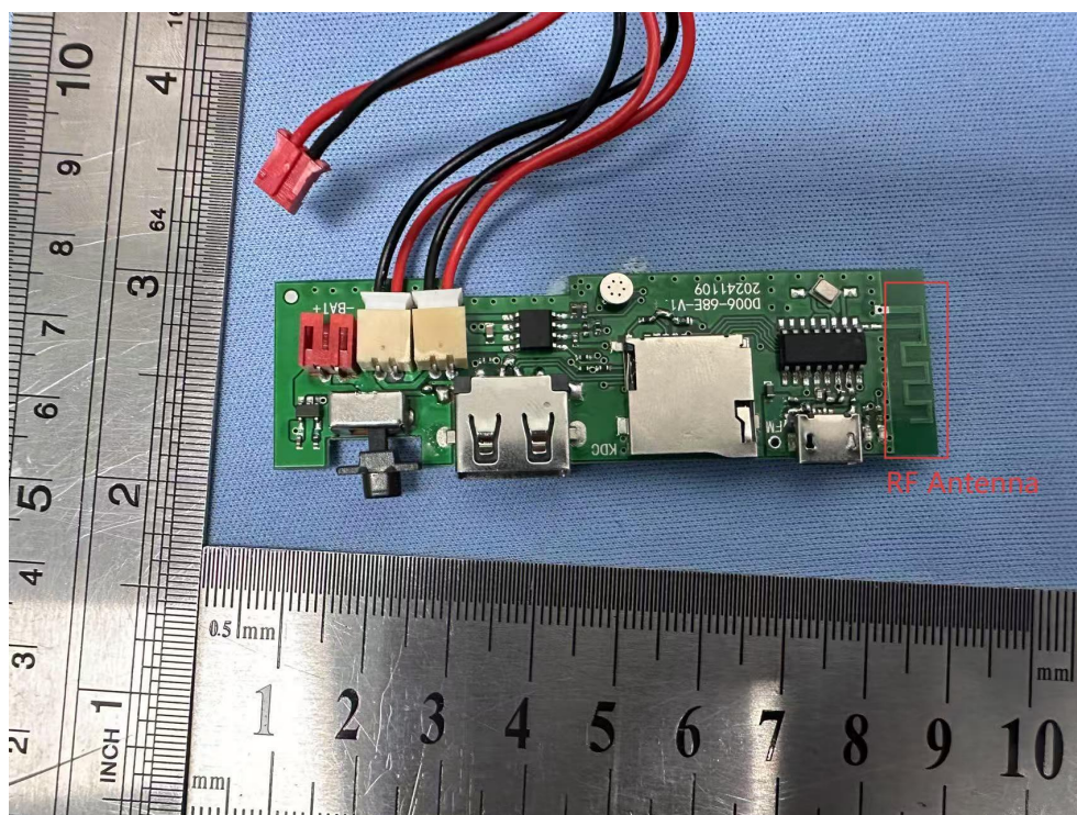
Internal Photos
