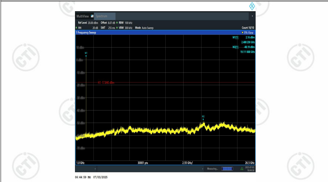
BLE_2M-Ant1-2480-1000~26500-PASS
