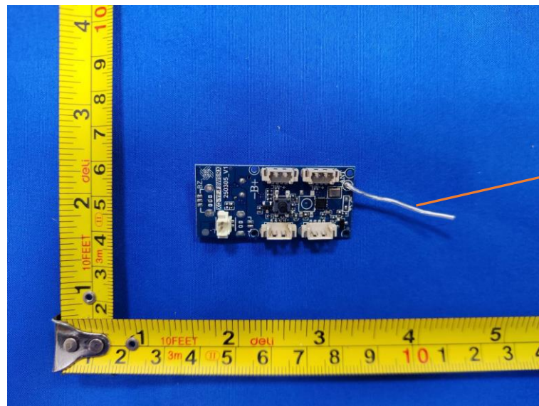
2.4G Receiving Antenna
