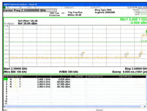
Band-edge Emission
