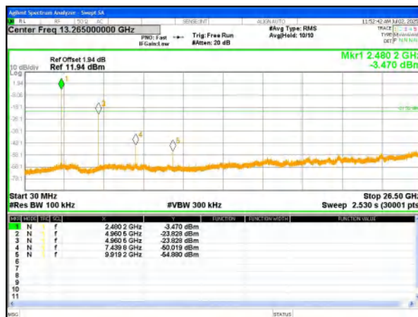
Spurious Emissions
